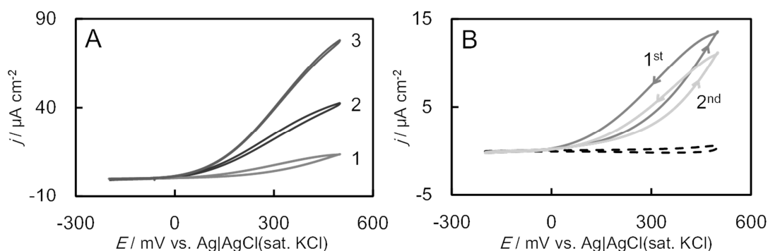
Figure 1. (A): CVs of fructose oxidation catalyzed by FDH adsorbed on (1) MEtn-modified, (2) MEtOH-modified, and (3) bare Au electrode in the presence of 200 mM fructose.
