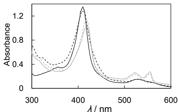
Figure 1. Absorption spectral change of FdhC solution in MacIlvaine buffer (pH 5.0). FdhC was fully oxidized by addition of potassium ferricyanide (solid black line). After then, FdhSL (dash black line), fructose (solid gray line) and sodium dithionite (dash gray line) were added in order.
