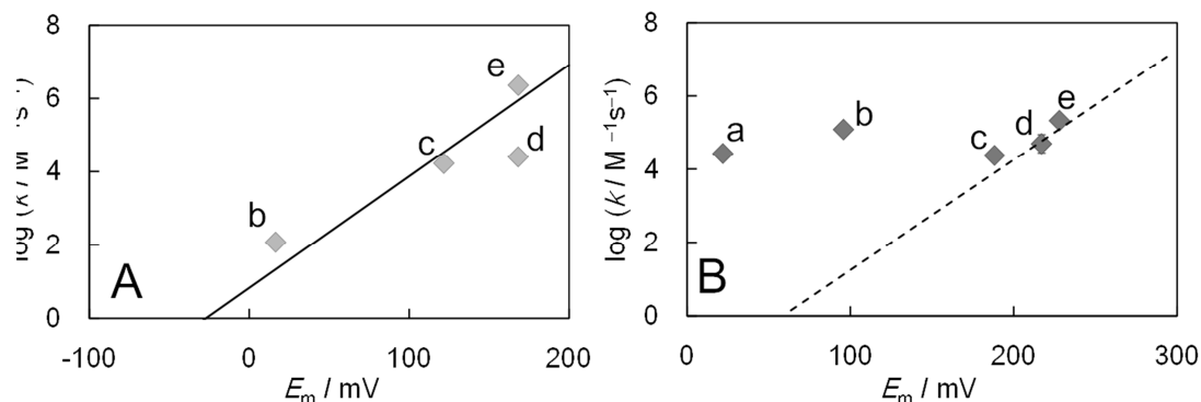
Figure 3. Bi-molecular rate constant ( k ) between the D-fructose-reduced enzymes ((A): FdhSL at pH 6.0 and (B): FDH at pH 5.0 in the presence of 1% TritonX-100) and p BQ derivatives as a function of the midpoint potential ( E_m ) of the quinones. The linear line in panel A indicates the linear-regression result: \log(k) = (30 \pm 1) \times E_m [\text{in mV}] + 0.83 \pm 1.3 . The electron acceptors used are: (a) 2,3-dimethoxy-5-farnesyl- p BQ ( Q_1 ), (b) 2,3-dimethoxy-5-methyl- p BQ ( Q_0 ), (c) phenyl- p BQ, (d) p BQ, and (e) 2,5-dichloro- p BQ. The broken line in panel B is a tentative LFER line with a slope identical with that of the regression line in Fig. 2A. Q_1 reacts with FdhSL, but the rate constant is too small to be evaluated by voltammetry.
