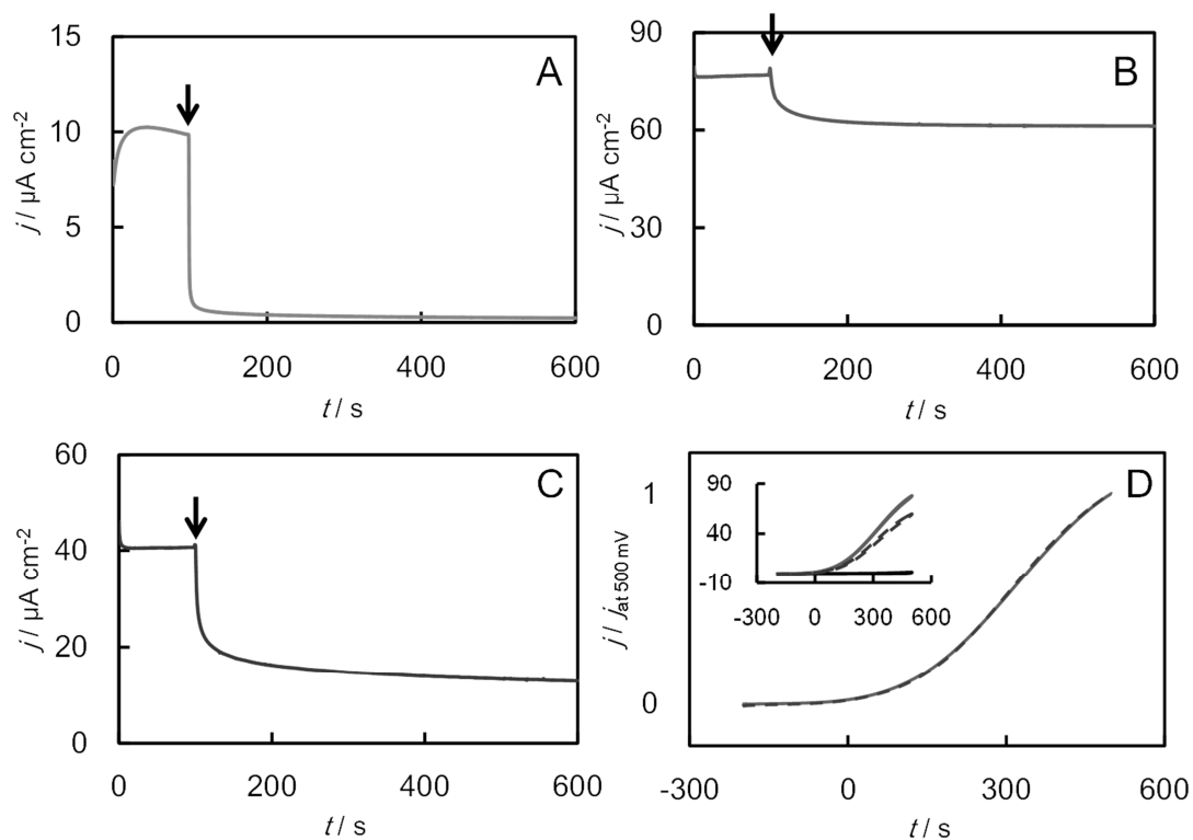
Figure 2. DET-type FDH-catalyzed current response in the presence of 200 mM fructose.
