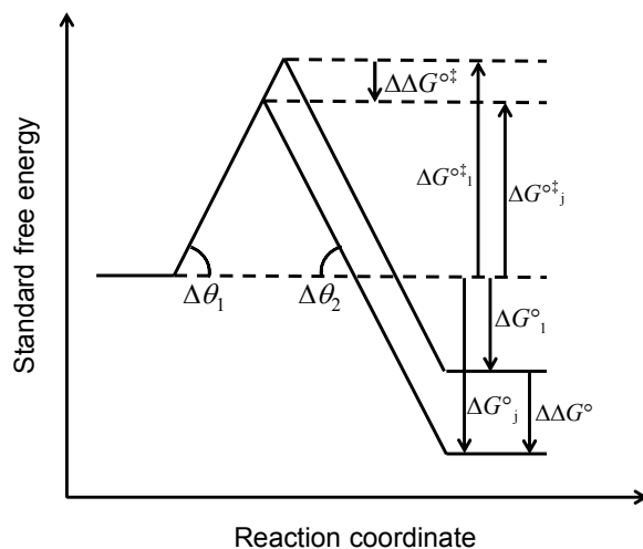
Figure 4. a schematic diagram of reaction energy map to explain linear free energy relationship
