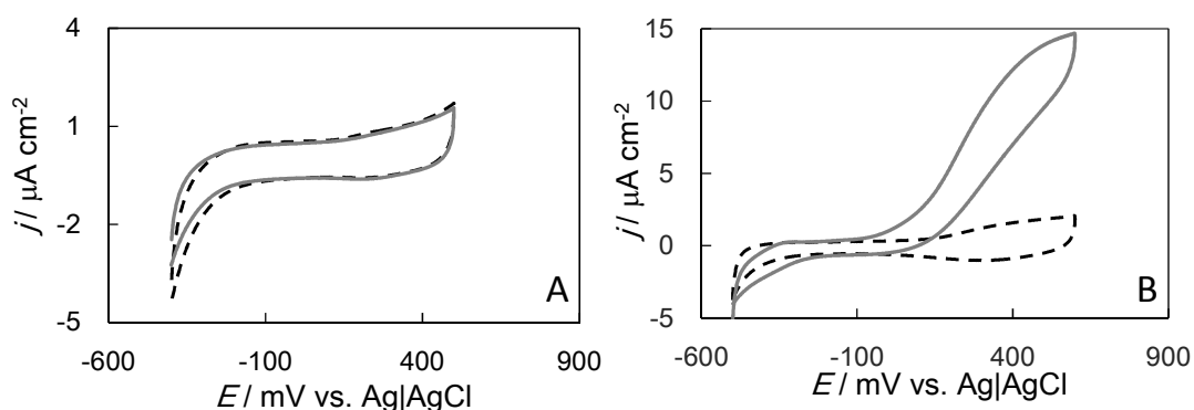
Figure 2. Cyclic voltammograms of FdhC (A) and the mixing solution of FdhSL and FdhC (B) in MacIlvaine buffer (pH 5.0) at v = 10 \text{ mV s}^{-1} and at GC electrode. Dash line: background current in the absence of enzyme, solid line: in the presence of FdhC (A), in the presence of FdhSL, FdhC and fructose (B).
