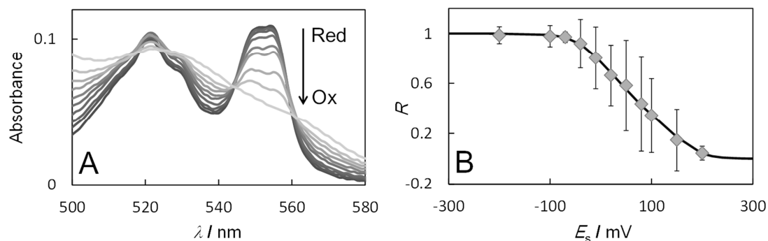
Figure 5. (A): Absorption spectral change of FDH solution in mediated spectroelectrochemical titration method without background subtraction. The mediators used for the bulk electrolysis were: 200 \mu\text{M} \text{Ru}(\text{NH}_3)_6\text{Cl}_3 , 200 \mu\text{M} (\text{NH}_4)_2\text{OsCl}_6 , 200 \mu\text{M} \text{Na}[\text{Fe}(\text{edta})] , and 100 \mu\text{M} \text{K}_3[\text{Fe}(\text{CN})_6] . The electrolysis solution were equilibrated electrochemically at -200, -100, -70, -40, -10, 20, 50, 80, 100, and 150 mV from (Red to Ox in tern). Measurements were carried out in McIlvaine buffer (pH 5.0) under anaerobic conditions at 25 °C. (B): Nernst analysis of the solution potential ( E_s )-dependence of the absorbance at 550 nm in Panel A. The error bars were evaluated by the Student t -distribution with a 90%-confidence level from 7 times of independent experiments. The solid regression curve was evaluated by a non-linear least-square method based on Eqs. (14) and (15).
