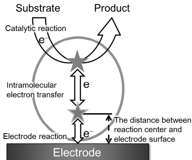
Figure 1. Schematic model of the ideal direct electron transfer pathway
