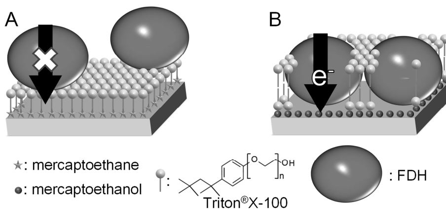
Figure 5. The proposed scheme of the adsorption of FDH and Triton® X-100 at (A) hydrophobic and (B) hydrophilic electrodes.
