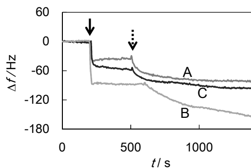
Figure 4. Frequency changes on the addition of 1% Triton® X-100 (at the solid arrow) and FDH (at the dashed arrow) at (A) MEtn-modified, (B) MEtOH-modified, and (C) bare Au electrodes.
