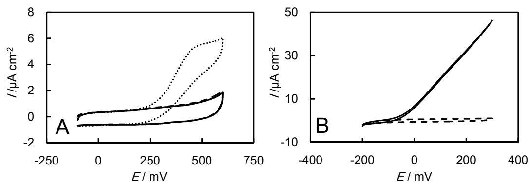
Figure 1. (A): Cyclic voltammograms (CVs) of fructose oxidation (0.2 M) catalyzed by (A) FdhSL (pH 6.0) and (B) FDH (pH 5.0) at \nu = 10 \text{ mV s}^{-1} and at an Au electrode. Dash line: fructose only, solid line: enzyme + fructose, dotted line: enzyme + p BQ + fructose.
