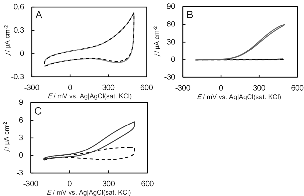
Figure 3. CVs of fructose oxidation catalyzed FDH adsorbed on (A) MEtn-modified, (B) MEtOH modified, and (C) bare Au(111) electrodes in the presence of 200 mM fructose and 1% Triton® X-100. All CVs were performed at pH 5.0 and \nu = 10 \text{ mV s}^{-1} . The background CVs (in the absence of fructose) are given by the broken curves.
