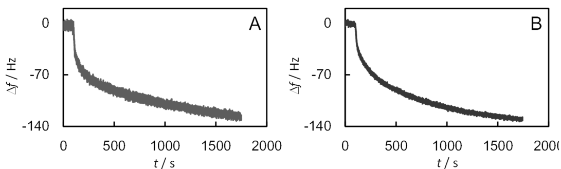
Fig. 6 Frequency changes on the adsorption of FDH in the absence of 1% Triton® X-100 at (A) MEtOH-modified and (B) bare Au electrodes.
