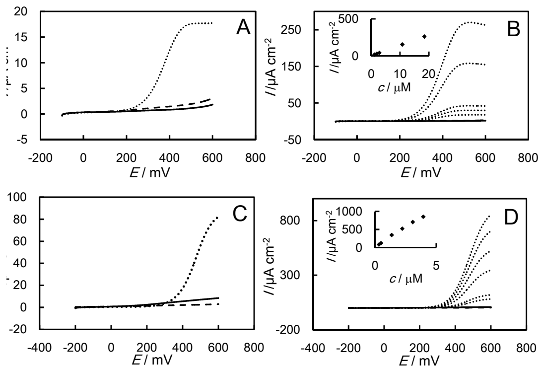
Figure 2. Linear sweep voltammograms of (A), (B) FdhSL and (C), (D) FDH at an Au electrode, scan rate = 10 \text{ mV s}^{-1} . The SLVs were measured in McIlvaine buffer (A), (B) pH 6.0 (as the optimum pH of FdhSL) and (C), (D) pH 5.0 containing 1% TritonX-100 (as the optimum pH of FDH) containing 0.2 M fructose. Dashed line: background current in the absence of FDH or FdhSL, solid line: in the presence of FDH or FdhSL, dotted line: in the presence of benzoquinone as a mediator at several concentrations. Inset at panel (B) and (D): The plots of the observed current density at 600 mV against the final concentration of benzoquinone.
