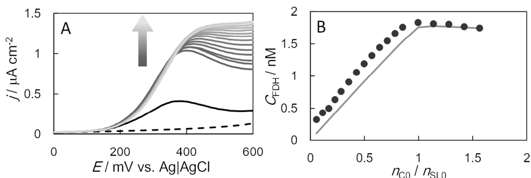
Figure 3. (A) Linear sweep voltammograms at an Au electrode, scan rate = 10 \text{ mV s}^{-1} . The SLVs were measured in McIlvaine buffer (pH 5.0) containing 1% TritonX-100 and 200 mM fructose. Dash black dash line: background current, Solid black line: in the presence of FdhSL and Q1 as a mediator, dash gray lines: in the presence of FdhC at several concentrations. (B) FDH concentration which was constructed by mixing FdhSL and FdhC as a function of the additional molar amount of FdhC to the initial molar amount of FdhSL ratio in panel A. The solid gray line was evaluated by a non-linear least-square method based on Eqs. (6) and (7).
