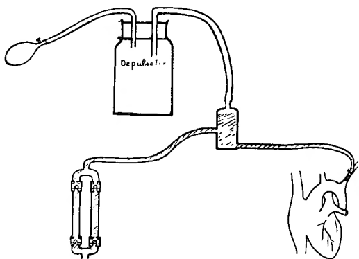
Fig. 1 Schematic illustration of depulsator system.
