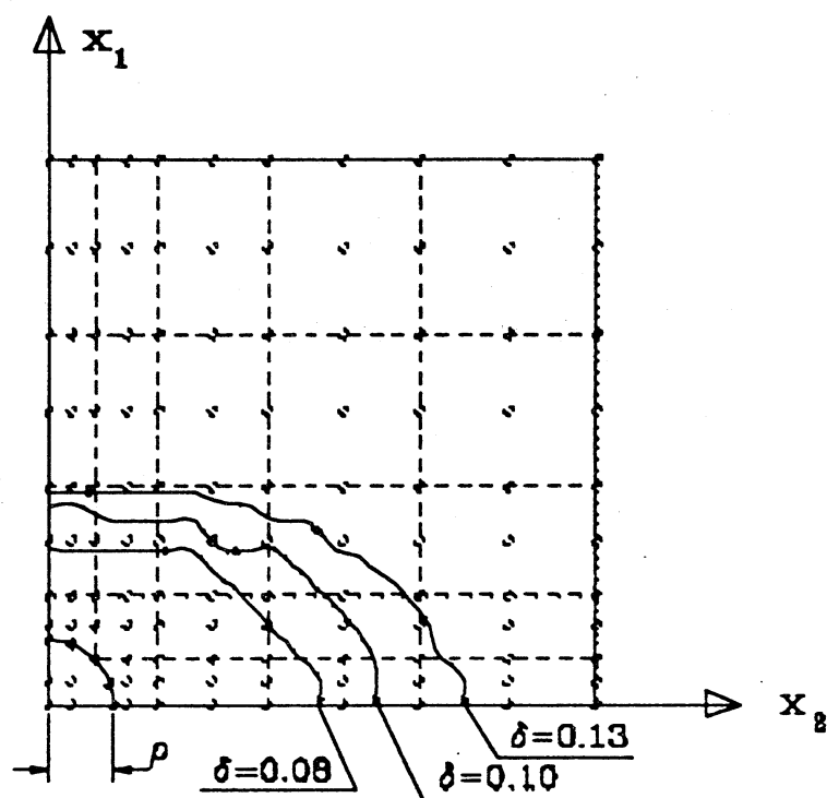
Figure 2 - Zones in adhesion and delaminated for \delta=0.08, 0.10 and 0.13\text{cm}
