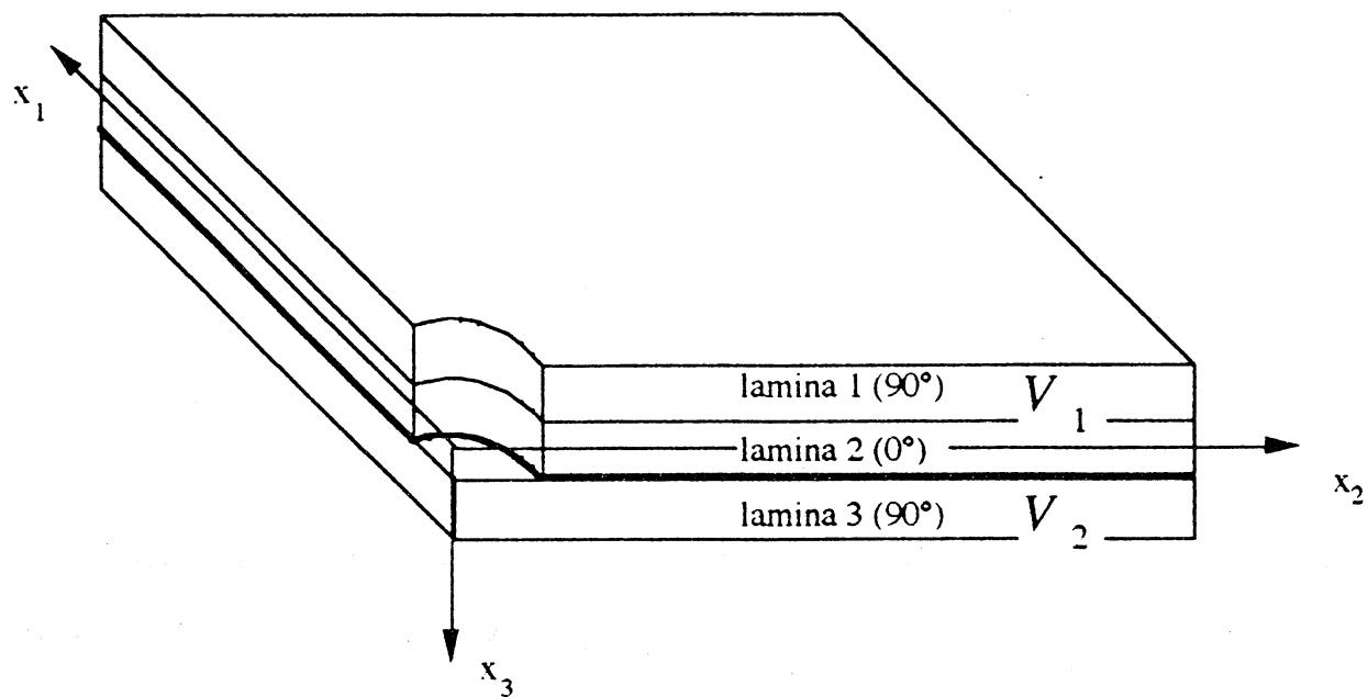
Figure 1 - A quarter of a cross-ply laminate with a hole in the first two laminae
