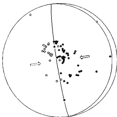
Fig. 3. Radiation pattern of P wave first motions projected on the lower half of the Wulff-net. solid circles : rarefactions, open circles : compressions. The arrows show the direction of the maximum pressure. The same explanations apply to Figs. 6, 7, 8, 9, 10, 13, 14, 15, 18, 19, 20, 21, 22.
