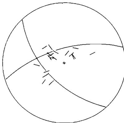
Fig. 16. S wave polarization angles.
