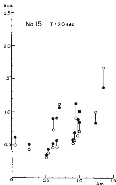
Fig. 5. Relation between the source amplitudes from observations and the theoretical amplitudes based on the solution for earthquake No. 15. Solid and open circles correspond to the unilayered and multilayered crustal models, respectively.
