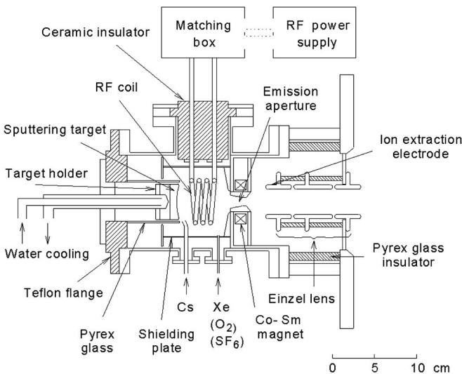
FIG. 2. Sputter-type heavy negative-ion source: rf-plasma sputter-type negative-ion source.
