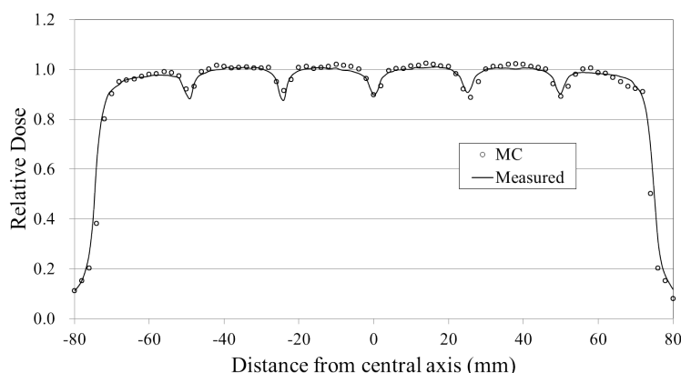
FIG. 7. T&G profiles as a function of distance from the central axis of simulated doses with a voxel resolution of 0.2 \times 0.2 \text{ cm}^3 , and measured doses.
