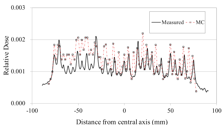
FIG. 6. Intra- and interleaf leakage profiles as a function of distance from the central axis of simulated doses with a voxel resolution of 0.2 \times 0.2 \times 0.2 cm 3 , and measured doses.
