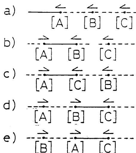
Fig. V-2. Stable part (solid line) on univariant reaction lines. Arrow shows radiating direction of univariant line from each invariant point. a) radiating in the same direction from three invariant point. b) - d) radiating in the same direction from two of three points, but in the opposite direction from the other.
