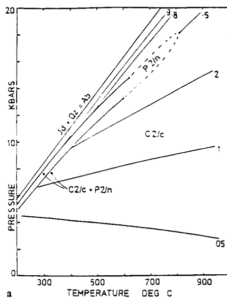
Fig. VI-3. Isopleths of \text{NaAlSi}_2\text{O}_6 with ordering to \text{P2/n} allowed for omphacites near to \text{Jd}_{50}\text{Di}_{50} (Holland 1983).
