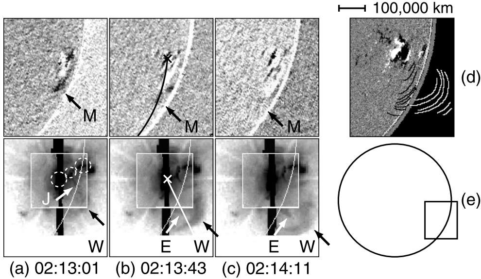
Fig. 1. Observed images on 2000 March 3, at NOAA AR 8882. Top panels of images (a)–(c) are H\alpha + 0.8 \text{ \AA} “running difference” images of a Moreton wave (black arrows “M”). Bottom panels of images (a)–(c) are negative soft X-ray images of an X-ray wave (black arrows “W”), ejecta (white arrows “E”) and a jet (white arrow “J”) taken with the Al-Mg filter. The images inside and outside the boxes are half-resolution ( 4''/91 ) and quarter-resolution ( 9''/82 ) images, respectively. The white dashed circles in image (a) show the bright regions in soft X-rays. The crosses and lines in image (b) are the flare site and measures of the wave, respectively. We assume that the brightest region in H\alpha is the flare site. Image (d) shows the wave fronts of the Moreton wave from 02:12:01 to 02:15:01 UT (black lines) and the X-ray wave from 02:13:01 to 02:14:11 UT (white lines) overlaid on the photospheric magnetic field observed at 01:35:02 UT. These wave fronts were determined visually. The box and circle shown in image (e) are the field of view of images (a)–(d) and the limb of the Sun, respectively.
