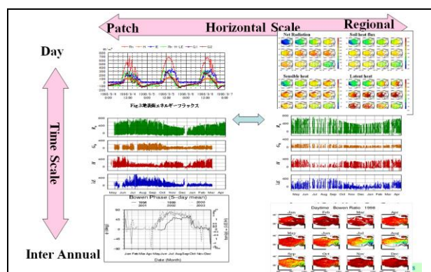
Figure 15 Combination of Surface observation (left row) and Satellite data retrieval (right row) enables regional and long-term estimate of surface fluxes.
