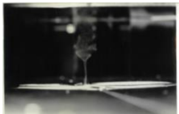
Figure 2 Tornado-like vortex generated in the tornado chamber with Radial_Reynolds'_Number = 2.6 \times 10^4 , and Swirl_ratio=0.4.
