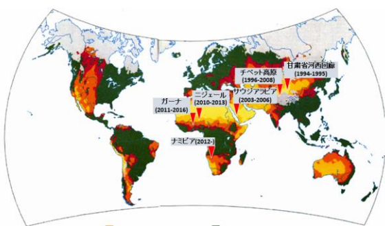
Figure 7 Footprint of my field research sites. The background map is quoted from UNEP 1991.
