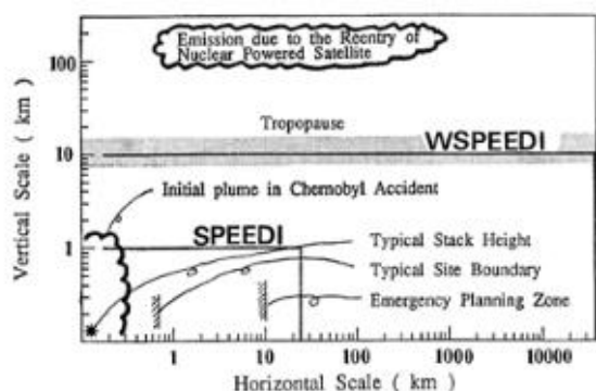
Figure 4 Spatial coverage of SPEEDI and WSPEEDI.
