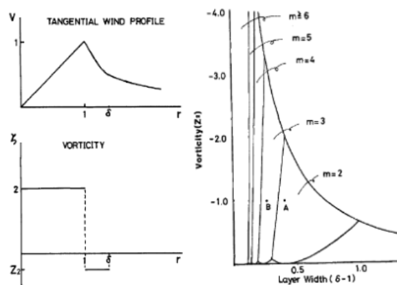
Figure 3 Model Profile of tangential wind and the vertical vorticity (left hand) and the stability diagram.
