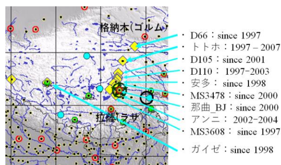
Figure 10 The deployment of project observation stations on the Tibetan Plateau.
