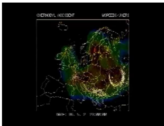
Figure 5 A snapshot of Chernobyl simulation movie. The resolution is rather poor since the media is S-VHS.
