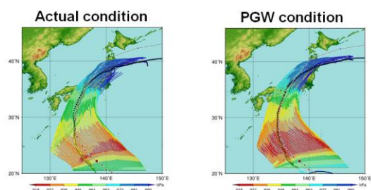
Figure 16 An example of Typhoon ensemble simulation. The worst case of Ise-bay typhoon was searched both for present and global warming environment.
