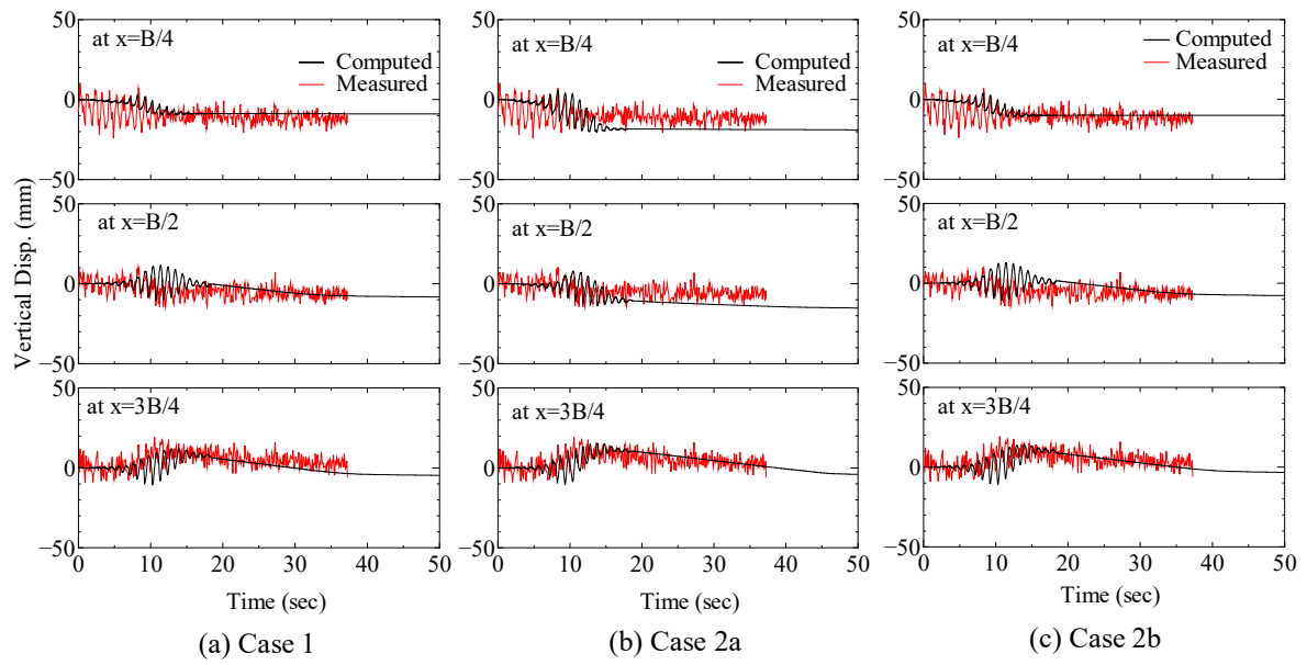
Figure 14 Computed time history of vertical displacement for KyU Centrifuge (LEAP-GWU-2015): (a) Case 1; (b) Case 2a; (c) Case 2b
