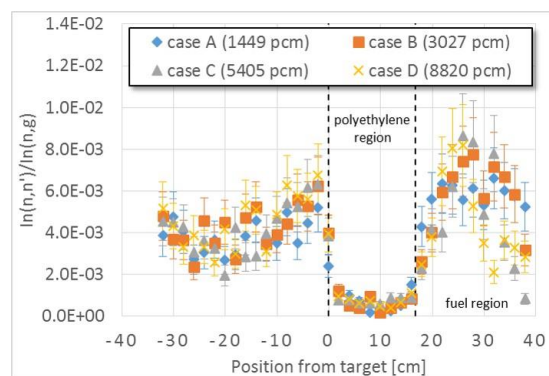
Fig. 3 Distributions of ^{115}\text{In}(n, n')/^{115}\text{In}(n, \gamma) ratio.
