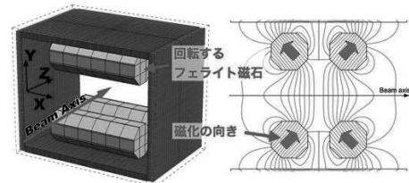
Fig. 2. Prototype correction magnet using a rotating ferrite.
