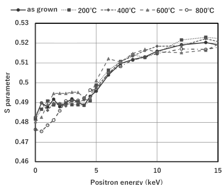
Fig. 3 S-E curves of annealed a-C:H films.
