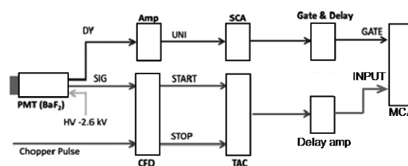
Fig. 5 Gate circuits for positron lifetime measurements.
