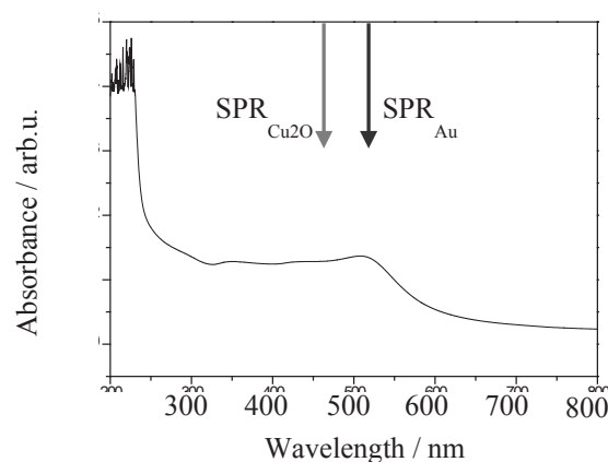
Fig.2. UV-vis spectrum of water solution including Ag, Au and Cu ions reduced by 8 MeV electron irradiation.
