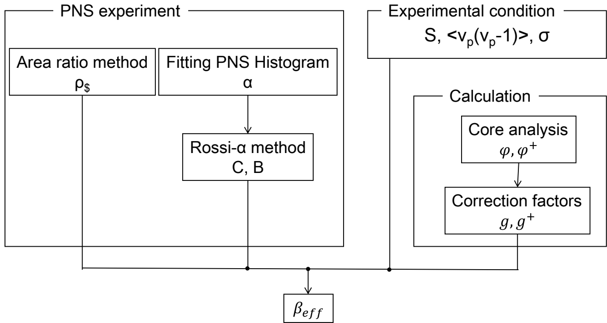
Fig. 3-1. Procedure for deduction of \beta_{\text{eff}} in PNS experiments.
