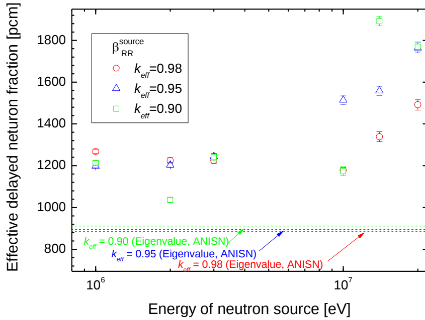
Fig. 4-5 Distribution of \beta_{RR}^{source} along to the energy of the neutron source at the core boundary as a spherical shell source.
