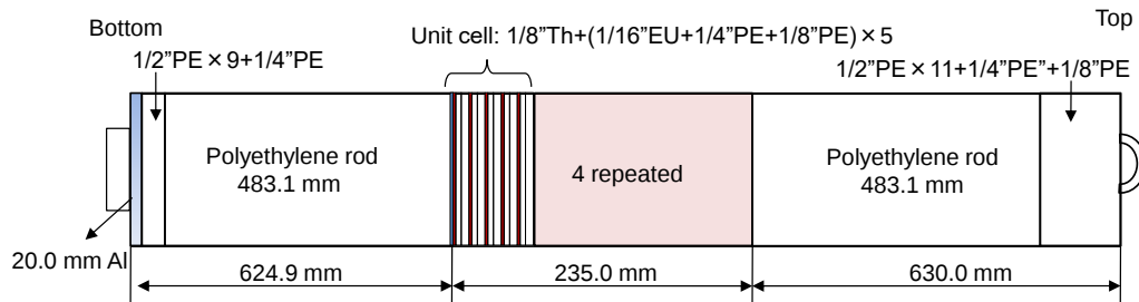
Fig. 2-2(c) Schematic detail of fuel rod "Th" (Th-HEU-5PE core) shown in Figs. 2-2(a) and 2-2(b).
