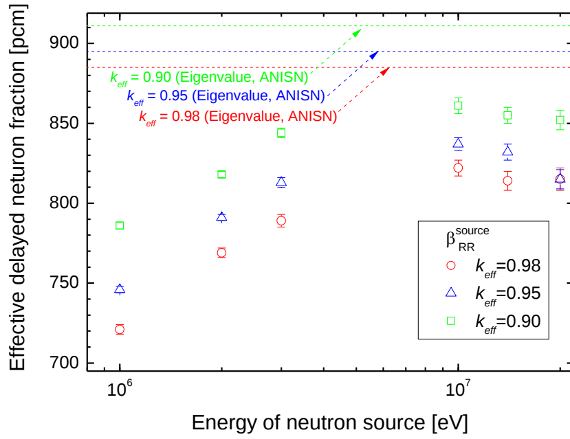
Fig. 4-4 Distribution of \beta_{RR}^{source} along to the energy of the neutron source at the core center as a point source.
