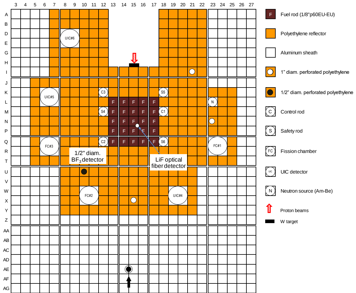
Fig. 3-3(a) Top view of 1/8" P60EU-EU(3) core for the measurement of \beta_{\text{eff}} with spallation neutrons in Cases B-I to B-III.
