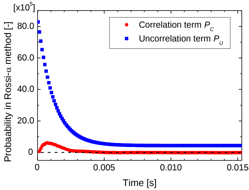
Fig. 3-5 Correlated and uncorrelated probabilities of fiber detector in Case B-I by Rossi- \alpha method in PNS experiments.
