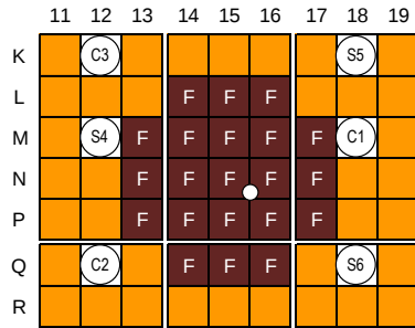
Fig. 3-3(b) Fuel substitution pattern I in 1/8" P60EU-EU(3) core for Cases B-IV to B-V. Fig. 3-3(c) Fuel substitution pattern II in 1/8" P60EU-EU(3) core for Cases B-VI to B-VII.
