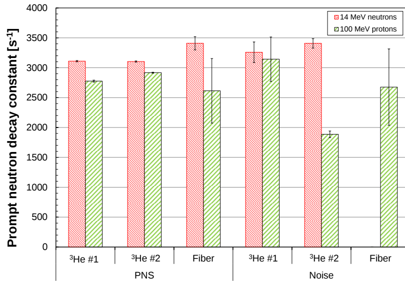
Fig. 2-4 Measured results of the prompt neutron decay constant \alpha 1/s by the PNS fitting method and the Feynman- \alpha method.
