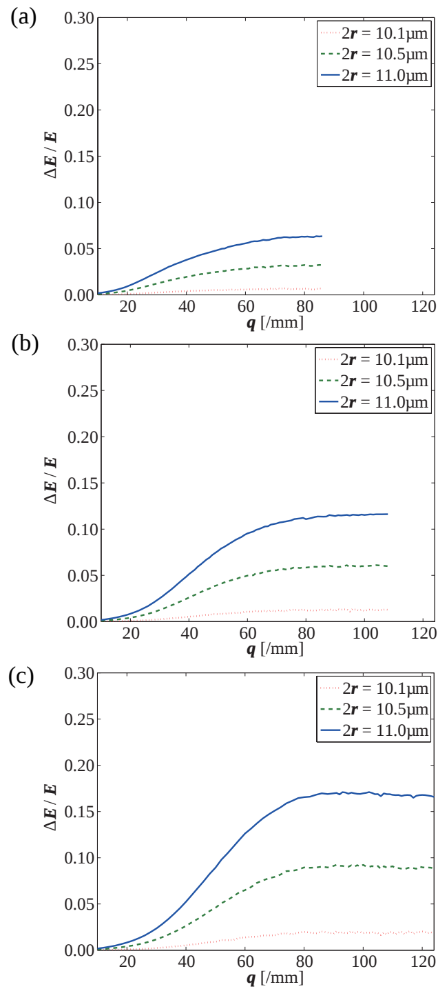
Figure 3.16: Normalized signal differences \Delta E/E , as function of various q , for 3 different b of 1000 \text{ s/mm}^2 (a), 2000 \text{ s/mm}^2 (b) and 3000 \text{ s/mm}^2 (c), when g=400 \text{ mT/m} .
