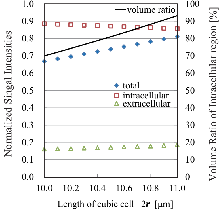
Figure 4.2: Normalized signal intensities E as function of 2r for b-values of 1000 \text{ s/mm}^2 and \Delta of 45.05 \text{ ms} , when g=25\sqrt{3} \text{ mT/m} ; total signal intensities (♦), intracellular ones (□), extracellular ones (△), and intracellular volume ratio(—).
