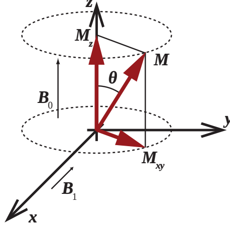
Figure 2.3: Net magnetization M can be divided into two components M_{xy} in x - y plane and M_z along z -axis in rotating coordinate systems.
