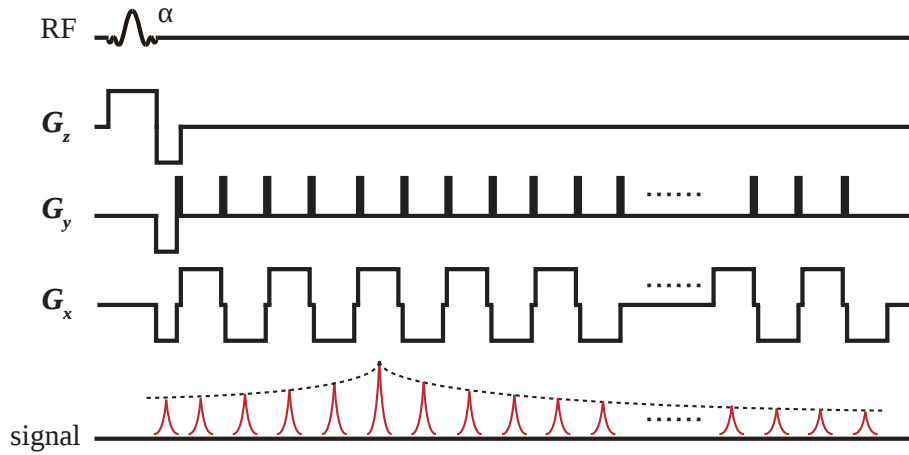
Figure 2.11: Pulse sequence of echo planar imaging.
