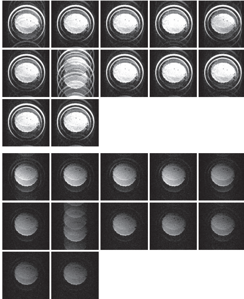
Figure 3.10: MR images of slices including capillary plate with capillaries of 10\ \mu\text{m} in diameter while b was fixed to 2000\ \text{s}/\text{mm}^2 . The first half of images are MR images without MPG and the others are those with MPG applied along both x - and y - axis. The q was set to 25, 30, 35, 40, 45, 50, 55, 60, 65, 70, 75 and 80 /\text{mm} in order from left upper side.
