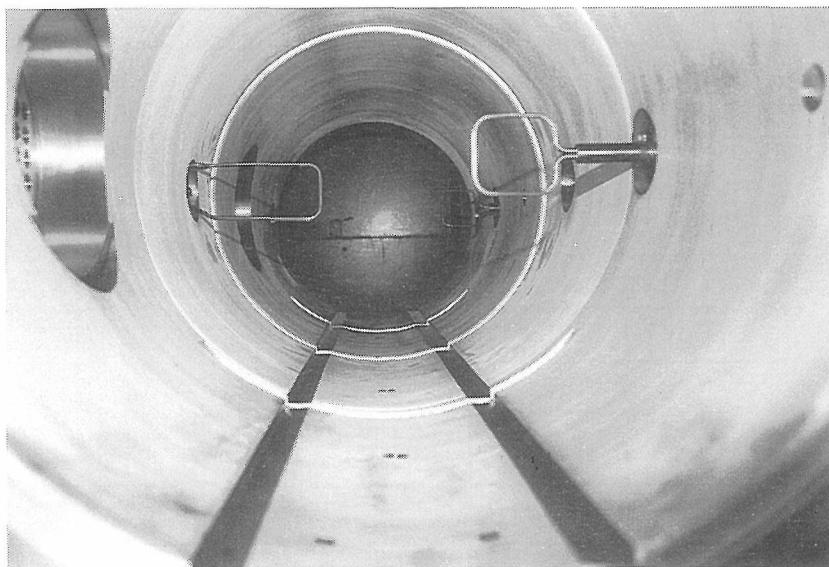
Photo. 2, Interior view of 33.3 MHz RFQ cavity.
