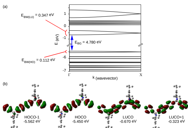
Figure 4. (a) Energy band diagram and (b) selected COs of polymer 1 . Hydrogen atoms are omitted for clarity.
