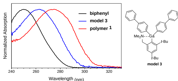
Figure 2. UV-vis absorption spectra of 1.0 \times 10^{-4} \text{ M} biphenyl, model 3 and polymer 1 in \text{CHCl}_3 solution.
