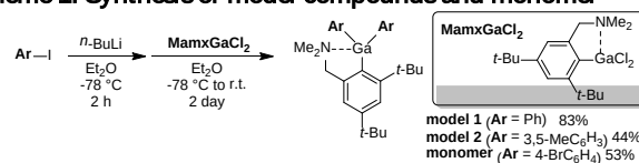
Scheme 1. Synthesis of model compounds and monomer
