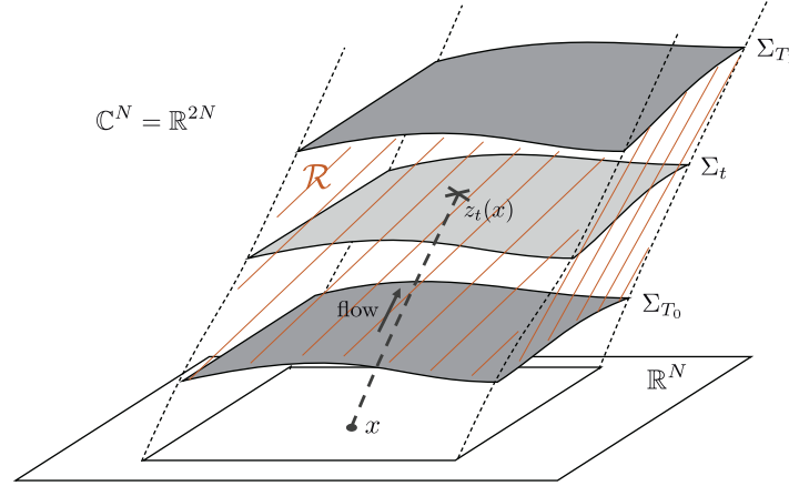
Fig. 1. The worldvolume \mathcal{R} (shaded region) embedded in \mathbb{C}^N = \mathbb{R}^{2N} .
