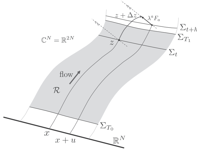
Fig. 7. A transition passing over the boundary at T_1 .
