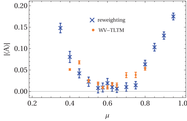
Fig. 9. Average phase factors \langle A \rangle = \langle e^{-i \text{Im} S(x)} \rangle_{\text{rewt}} from the naive reweighting method (blue) and the average reweighting factors \langle A \rangle = \langle A(z) \rangle_{\mathcal{R}} from the WV-TLTM (orange). The estimation range [\hat{T}_0, \hat{T}_1] in the WV-TLTM is set to that for the chiral condensate (see Table 1).
