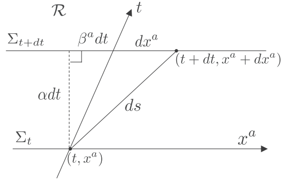
Fig. 3. Geometrical meaning of the ADM parametrization. \alpha dt is the geodesic distance from a point \xi = (t, x^a) on \Sigma_t to the surface \Sigma_{t+dt} . \beta^a dt shows that the time axis t is tilted with respect to the normal of \Sigma_t by this amount in the x coordinates. \gamma_{ab} is the induced metric on \Sigma_t . The geodesic distance ds between two points \xi = (t, x^a) and \xi + d\xi = (t + dt, x^a + dx^a) is then obtained from the Pythagorean theorem as in Eq. (43).
