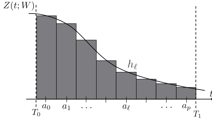
Fig. 6. Estimating Z(t; W) from \{h_\ell\} .
