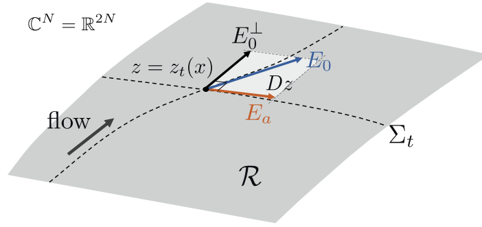
Fig. 4. E_0^\perp and the volume element.
