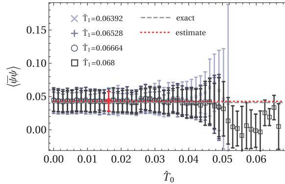
Fig. 10. Estimates of \langle \bar{\psi} \psi \rangle at \mu = 0.575 with various \hat{T}_0 and \hat{T}_1 . The red filled box is the point taken from a plateau, giving the estimate 0.043(15) (shown by the dotted line). The exact value ( = 0.041 ) is shown by the dashed line.
