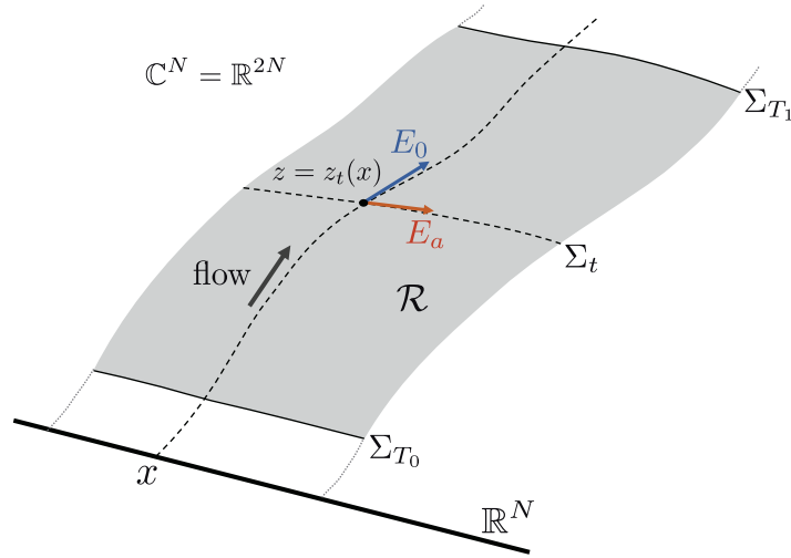
Fig. 2. A basis of T_z \mathcal{R} , \{E_\mu\} = \{E_0, E_a\} . \mathcal{R} is drawn one dimension less than in Fig. 1.
