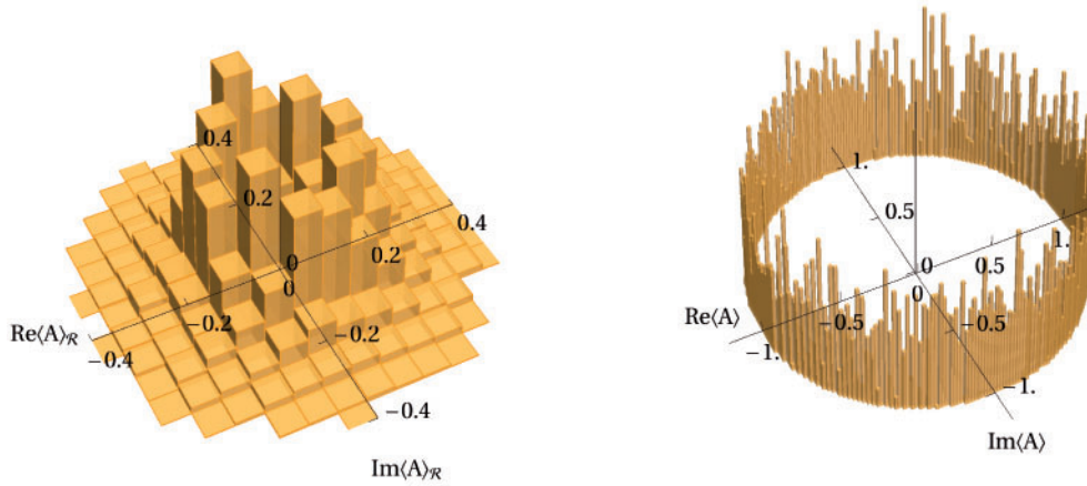
Fig. 12. (Left) Histogram of A(z) = \alpha^{-1}(z) e^{i\varphi(z) - i \text{Im} S(z)} obtained from the WV-TLTM. (Right) Histogram of the phase factor e^{i\varphi(z) - i \text{Im} S(z)} obtained from the reweighting. Both figures are at \mu = 0.575 .
