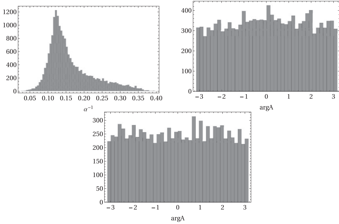
Fig. 13. (Top) Histograms of the modulus |A(z)| = \alpha^{-1}(z) and the phase \arg A(z) = \varphi(z) - \text{Im } S(z) from the WV-TLTM. (Bottom) Histogram of the phase from the reweighting method. All figures are at \mu = 0.575 .
