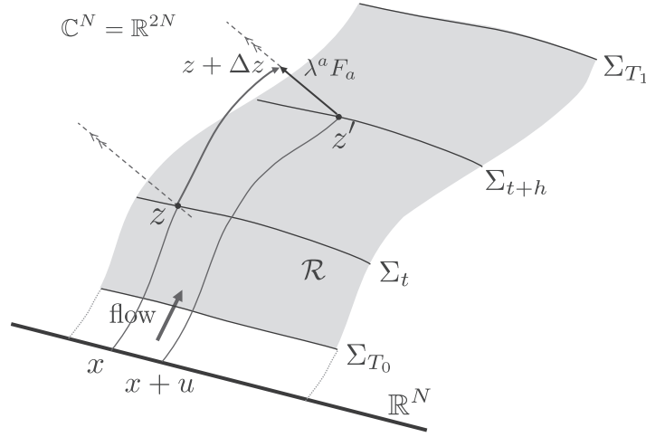
Fig. 5. Finding z' = z(\xi + \varepsilon) = z_{t+h}(x + u) on \mathcal{R} from z = z(\xi) = z_t(x) \in \mathcal{R} .
