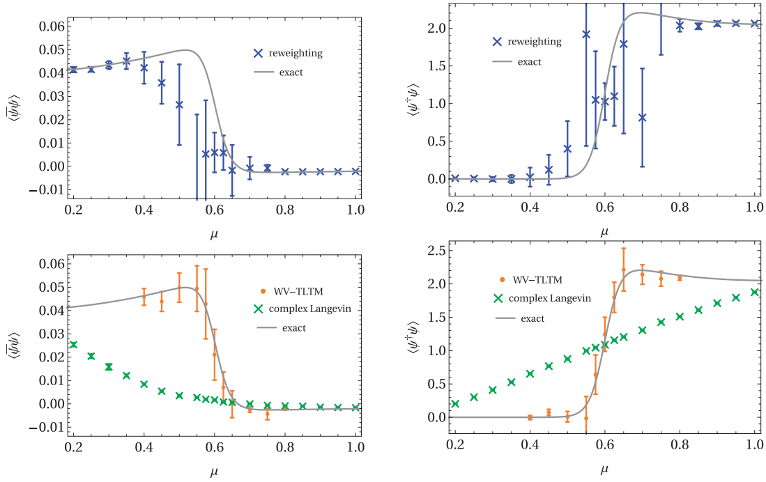
Fig. 11. (Left) The chiral condensate. (Right) The number density. The top panels are the results from the reweighting method, and the bottom panels are from the WV-TLTM and the complex Langevin method.
