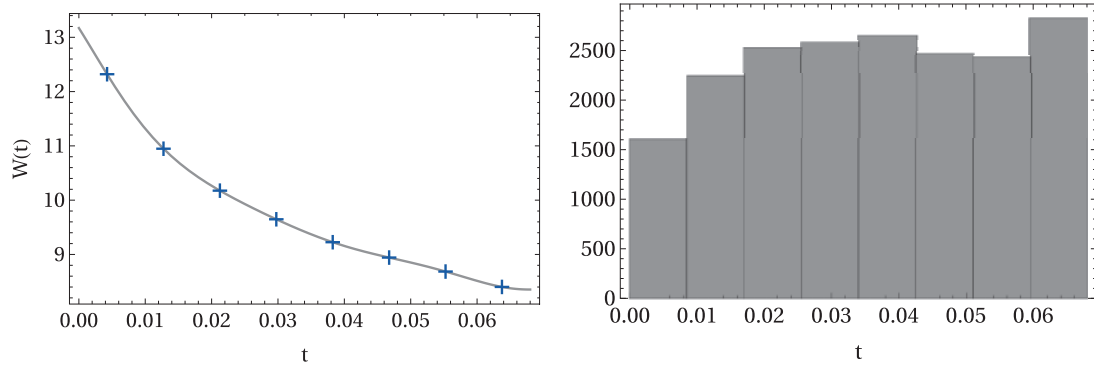
Fig. 8. (Left) Final \{W_\ell\} and its polynomial fit W(t) . (Right) Final histogram of t . Both figures are at \mu = 0.575 .
