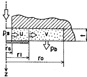
Fig. c. Measurement of \tau .
