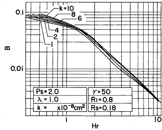
Fig. 6. Effect of permeability coefficient on B .
