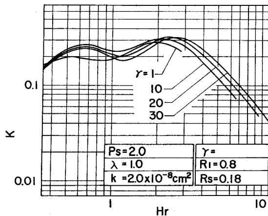
Fig. 7. Effect of permeability ratio on K , (i).
