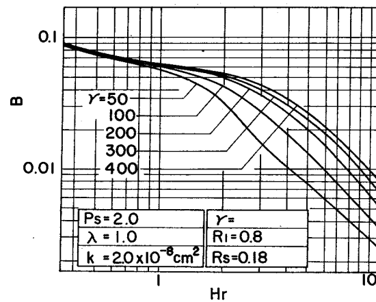
Fig. 10. Effect of permeability ratio on B , (ii).
