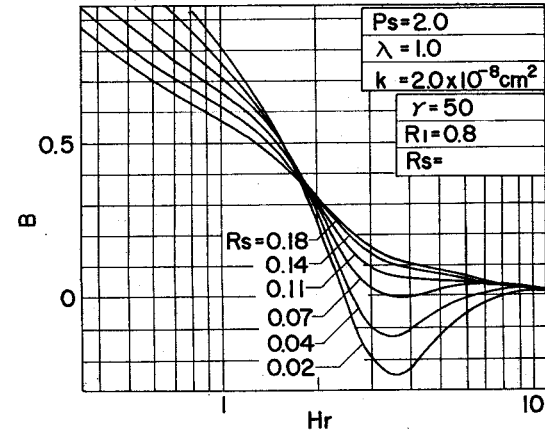
Fig. 14. Effect of R_s on B .
