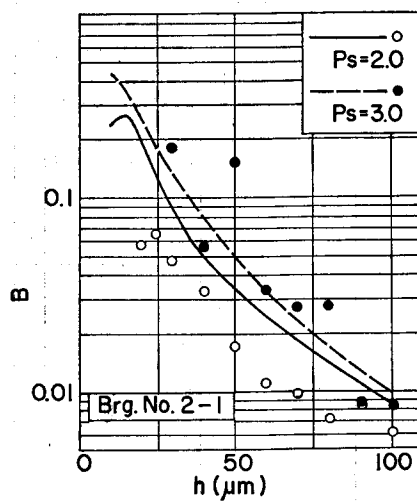
Fig. 31. Damping coefficient vs. bearing gap, (i).
