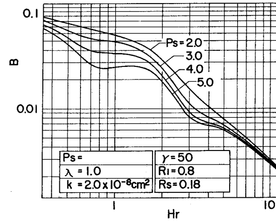
Fig. 4. Effect of supply pressure on B .
