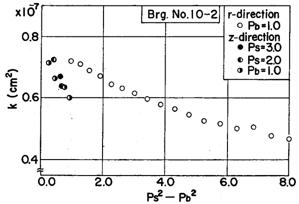
Fig. 22. Measured permeability coefficient, (iv).
