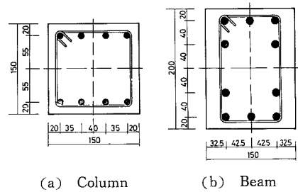
Fig. 2 Cross section of test specimen.
