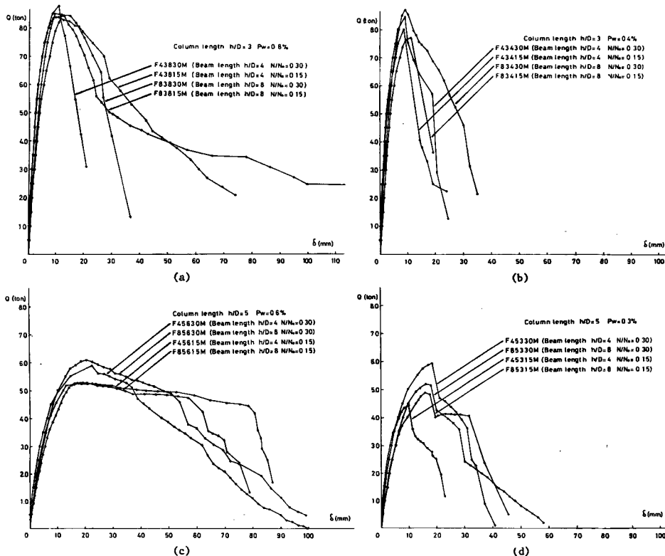
Fig. 8 Shear-deflection relationships for monotonic loading.
