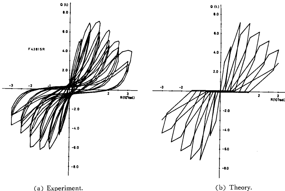
Figs. 21 Hysteresis loop obtained from simplified model.
