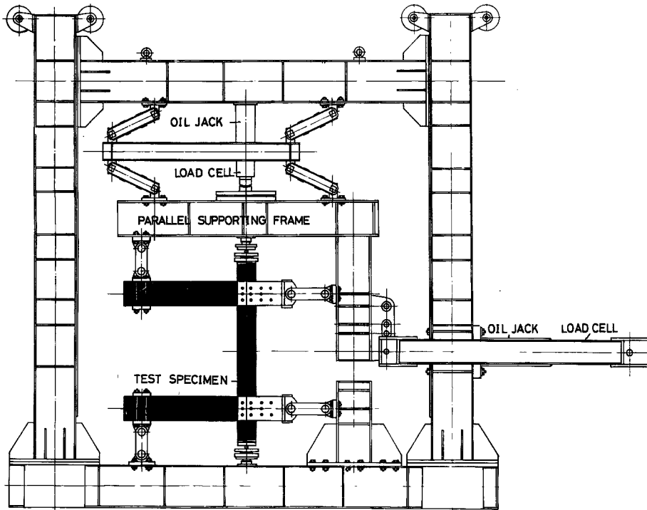
Fig. 4 Loading apparatus.
