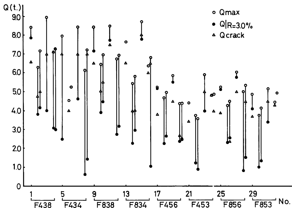
Fig. 10 Measured maximum and minimum shear.
