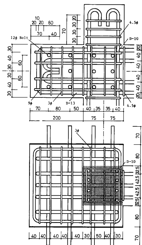
Fig. 3 Detail of beam-to-column connection.
