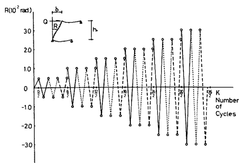
Fig. 7 Loading program.
