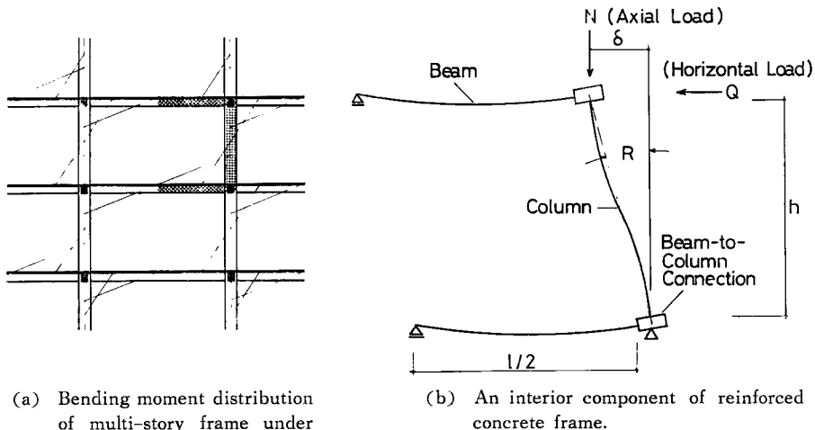
Fig. 1 Idealized model of interior subassembly.
