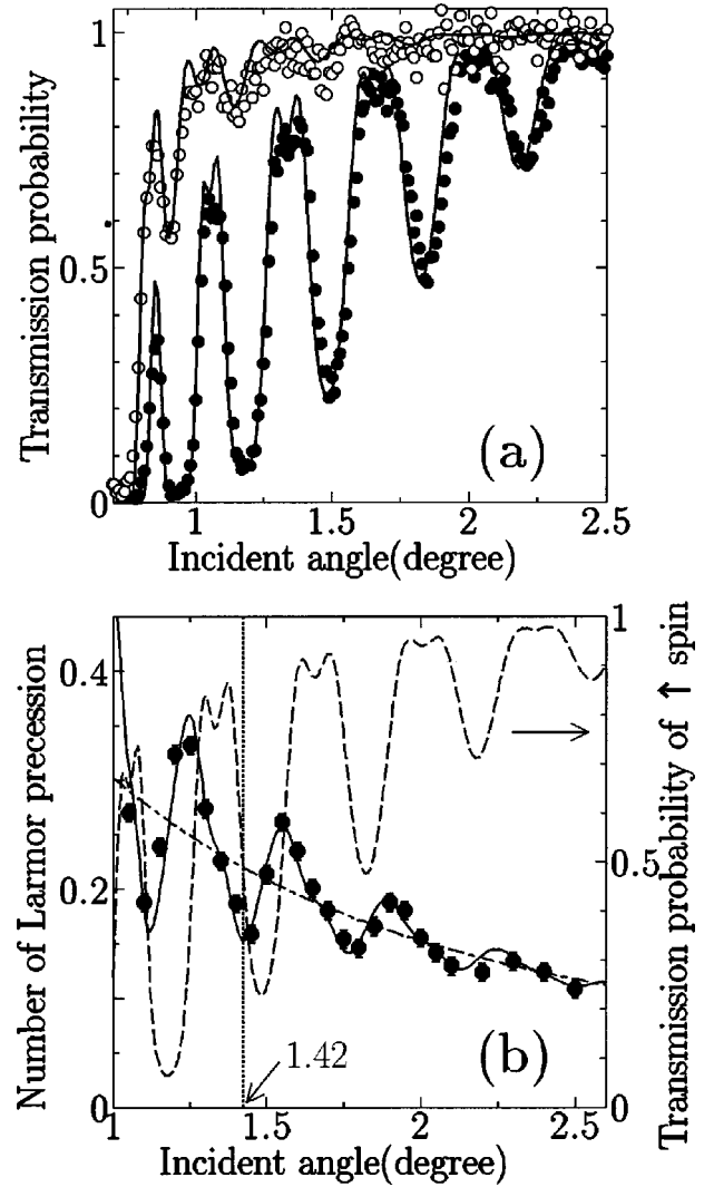
FIG. 7. (a) Transmission probabilities of \uparrow and \downarrow spin neutrons through the [PA(10 \text{ nm})-Ge(80 \text{ nm})]^2 -PA(10 nm) Fabry-Perot resonator as a function of the incident angle. (b) The spin precession of neutrons due to the Fabry-Perot resonator as a function of the incident angle.
