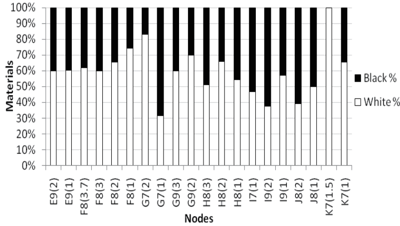
Fig.6 Materials distribution at different height for Case 18°
