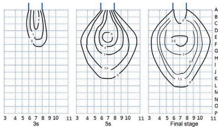
Fig. 4 Three stages of debris formation for case
