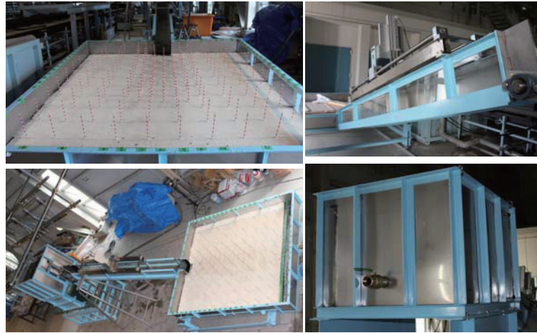
Fig. 1 The debris flow experimental model
