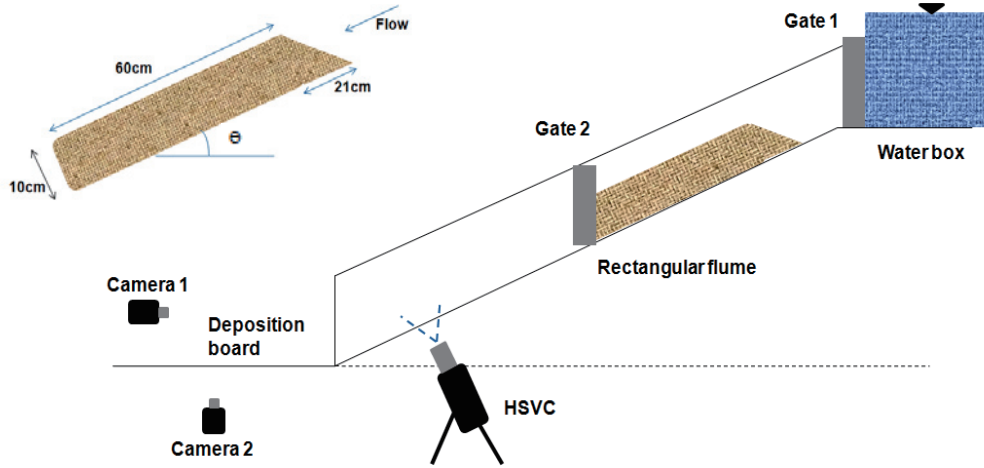
Fig. 2 The diagram of the experimental set-up
