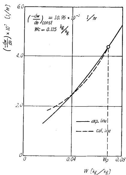
Fig. 11. Comparison between experimental and calculated drying rate.
