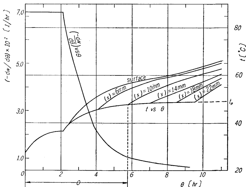
Fig. 6 (a). Temperature distribution curves. (Run No. Ac-7, Acricon (42~60#) t_a=71.0^\circ\text{C} , H_a=0.0113 , V_a=1.8 m/sec, L=0.03 m)
