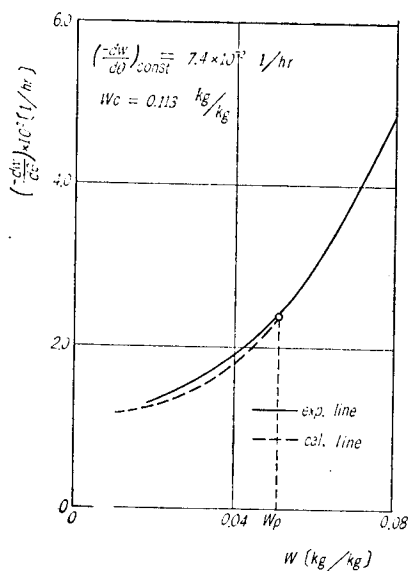
Fig. 11. Comparison between experimental and calculated drying rate.
