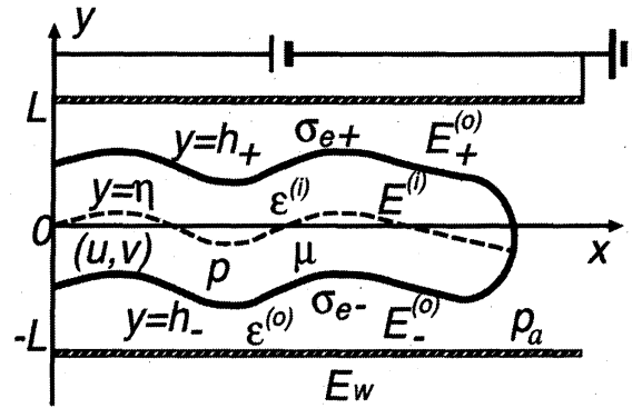
Figure 1: A two-dimensional planar liquid jet between two parallel sheaths on which an external electric field is imposed.
