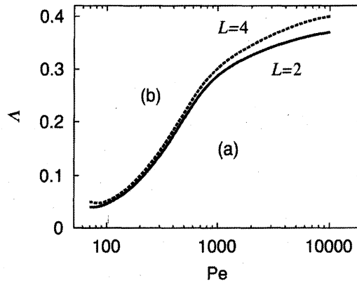
Figure 3: Critical curves discriminating the surface tension dominant mode referred to as (a) and the electric force dominant mode as (b) in (\Lambda, Pe) space when L = 2 (solid line) and 4 (broken line).
