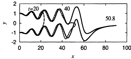
Figure 4: Evolutions of the jet surfaces for the fluctuation \eta = A \sin \omega t and v = A \omega \cos \omega t with A = 0.05 and \omega = \pi/5 when Pe = 100 , \Lambda = 0.1 .
