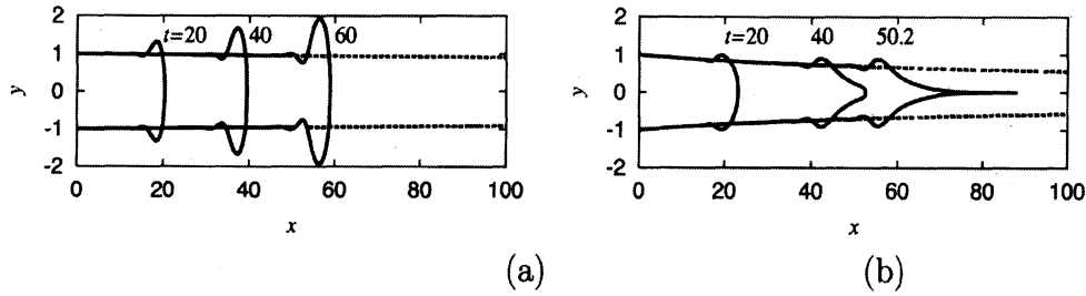
Figure 2: Evolutions of the profiles h_{\pm} for the symmetric mode, where Pe = 100 and \Lambda = 0.01 for the surface tension dominant mode in (a), while Pe = 100 and \Lambda = 0.1 for the electric force dominant mode in (b). On the other hand, the steady solutions are shown in the broken lines.
