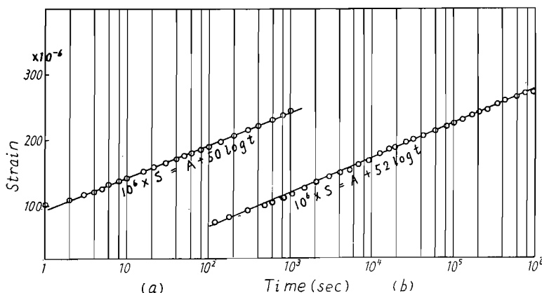
Fig. 5. Creep curves of lateral direction for Shōdoshima biotite granite under load of 1170 \text{ kg/cm}^2 , (a) short period test, (b) long period test.
