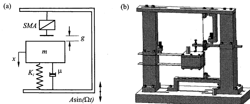
Figure 1: (a) Physical model of impact oscillator with SMA constraint [2]; (b) schematic of the impact oscillator where the secondary constraint is comprised of a stiff steel beam with a hinge supported by pseudoelastic wires.
