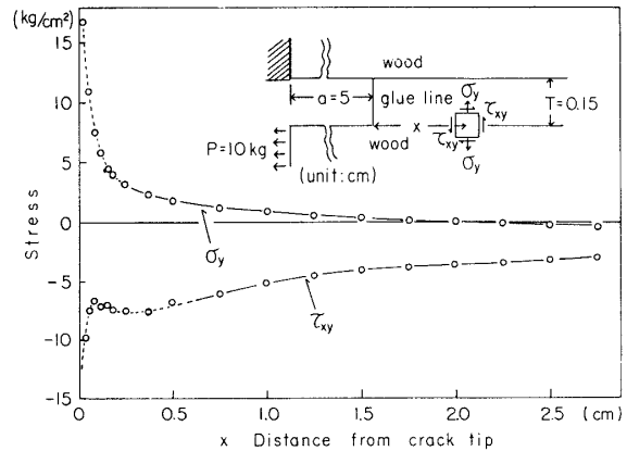
Fig. 11. Distribution of \sigma_y and \tau_{xy} along the interface between adhesive and center adherend.
