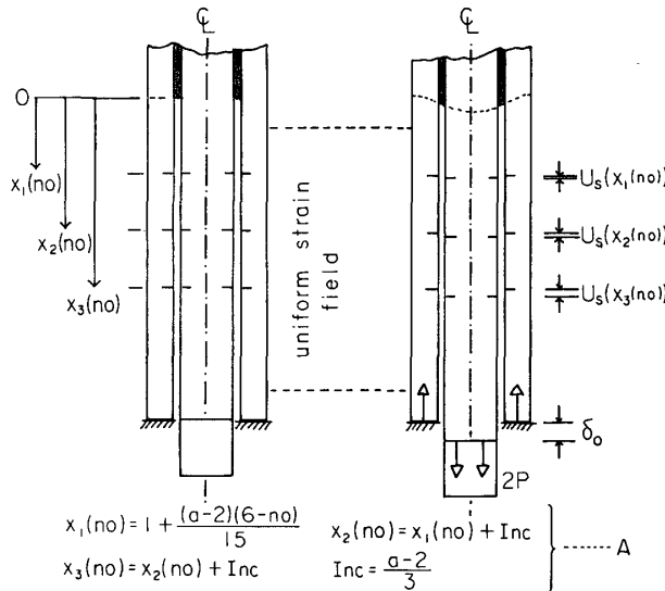
Fig. 5. Schematic diagrams of measurement of relative displacement.
