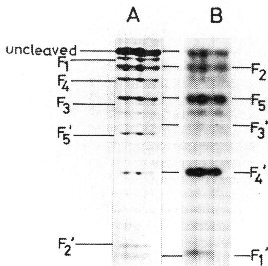
Fig. 38. Distribution of Fragments Incorporating ^{14}\text{C} over the Fragments Formed by Cleavage at Each One of the Five SH groups.
