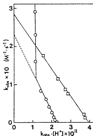
Fig. 9. k_{obs} vs. k_{obs} \cdot [H^+] Plot for the Reaction of SH2 with Iodoacetamide.
