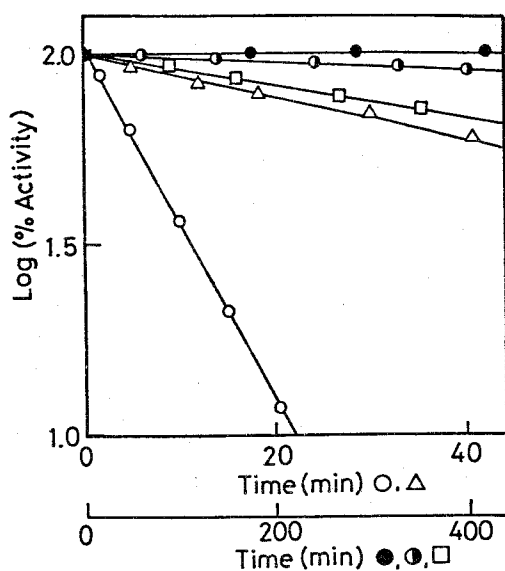
Fig. 17. Inactivation of Soybean \beta -Amylase by Disulfides in the presence of \text{Cu}^{2+} .
