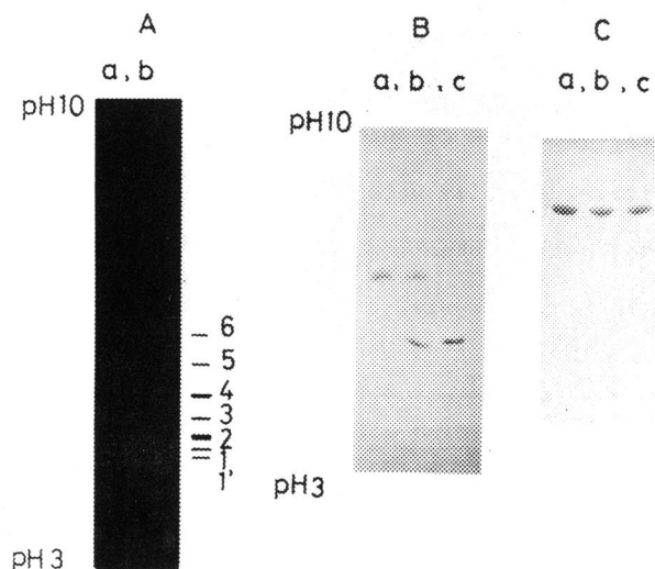
Fig. 5. A, Gel Isoelectric Focusing of Component 6 and the Extract of Defatted Soybean Meal. The gel was stained by activity. a, component 6; b, the extract of commercial defatted soybean meal.
