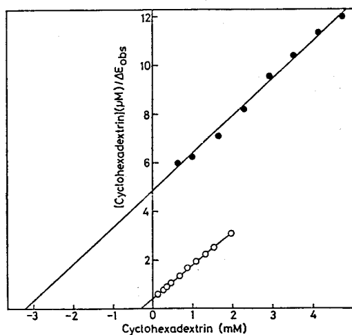
Fig. 25. Plots of [\text{cyclohexadextrin}]/\Delta\epsilon_{\text{obs}, 299 \text{ nm}} versus [\text{cyclohexadextrin}] for the Specific Difference Spectra of \beta -Amylase Produced by Cyclohexadextrin in the Presence of Maltose.
