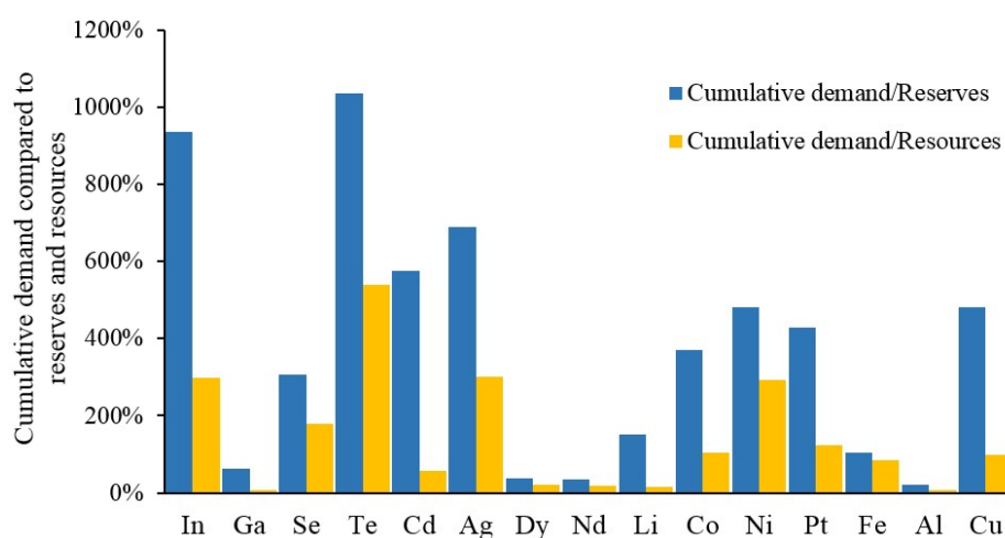
Figure 13. Cumulative demand from 2016 to 2060 compared to the reserves and resources in the case of 2DS-Ref.
