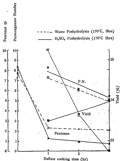
Fig. 5. Sulfate cooking.
