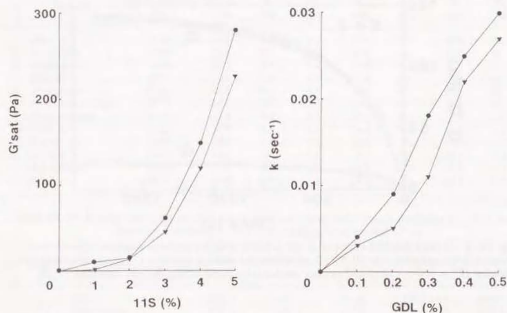
Fig. IV-3.(left) Dependence of saturated storage modulus G'_{\text{sat}} on the concentration of 11S globulin in the presence of 0.4 % GDL. ●, Enrei; ▼, Tsukuizairai.
