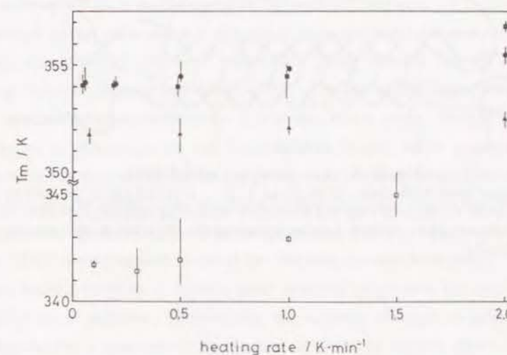
Fig. II-4. Dependence of gel melting points T_m on the heating rate.
