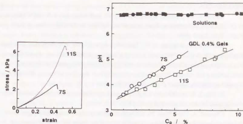
Fig. IV-28.(left) Typical stress-strain curves for a 7S (solid line) and an 11S (dotted line) globulin gels in the presence of 0.4 % GDL. Protein concentration: 4.0 %. Heated at 60 °C for 240 min in 7S, 60 min in 11S.
