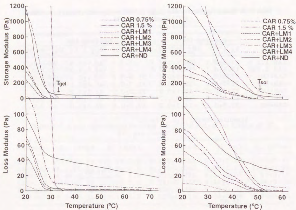
Fig. V-12.(left) Temperature dependence of storage and loss moduli for CAR and KGM mixtures in cooling process.
