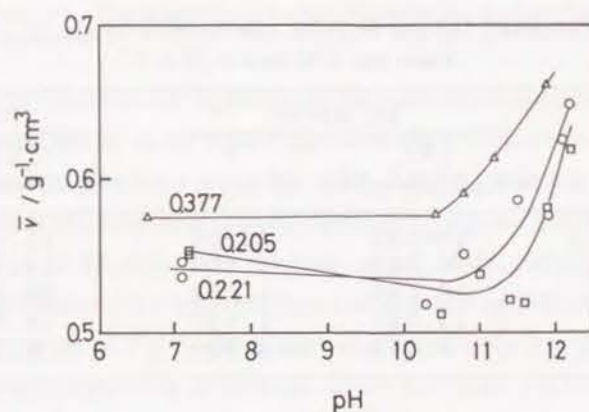
Fig. V-5. Dependence of apparent partial specific volume on pH at 25.0 ^\circ\text{C} . pH was adjusted by several alkali reagents: \circ , NaOH; \square , KOH; \Delta , \text{Ca}(\text{OH})_2 . The numbers beside each curve represent the concentration of konjac glucomannan in w/w%.
