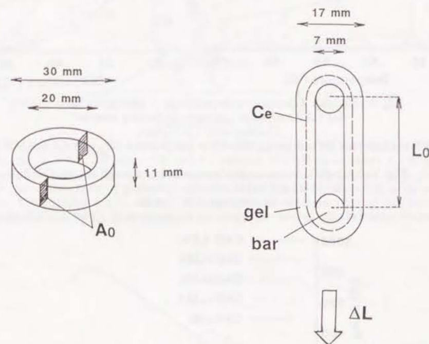
Fig. V-11. Shape and dimension of the gel ring for the tensile testing.
