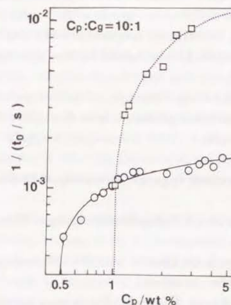
Fig. IV-30. Double-logarithmic plot of reciprocal gelation time t_0 against protein concentration C_p . The ratio of GDL to protein was 0.1 in both cases. Experimental data for 7S globulin (open circles) and for 11S globulin (open squares). Calculated curve for 7S using equation IV-4 with n=0.0192 , p=0.346 , C_0=0.479 and K=221 (solid line) and that for 11S with n=2.61 , p=0.341 , C_0=1.03 and K=271 (dotted line), respectively.
