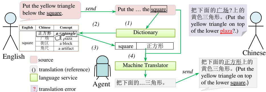
Figure 5.2: Interaction to handle inadequately translated phrase ( (1) check the feature that the word, “square”, has one-to-many dictionary results. (2) suggest the sender select the correct concept. (3) the sender chooses the target concept. (4) translate by the dictionary translator composite machine translator. )
