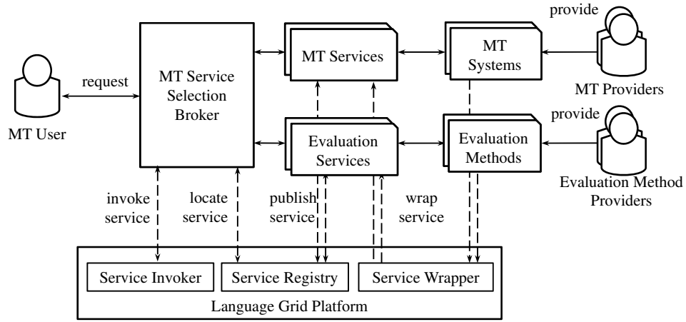
Figure 3.3: Service broker for selecting the best machine translation
