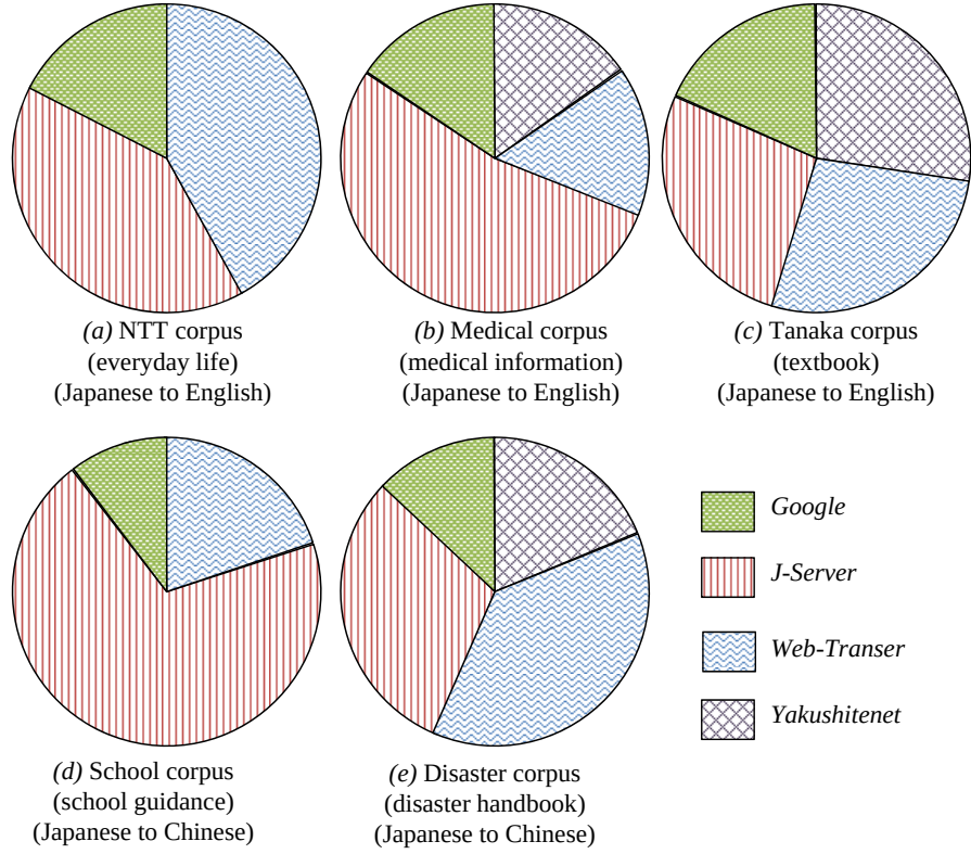
Figure 3.6: Percentage of best machine translations in each domain based on human score: adequacy
