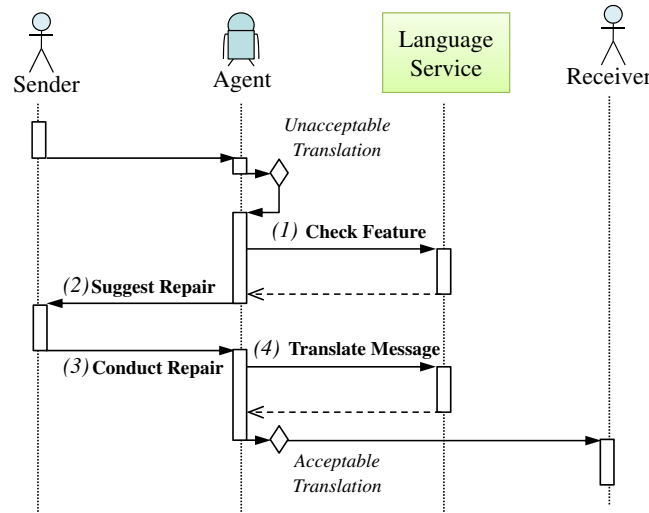
Figure 5.5: Four steps of the interaction process for one repair strategy ( (1) Check Feature, (2) Suggest Repair, (3) Conduct Repair (Sender), and (4) Translate Message. )
