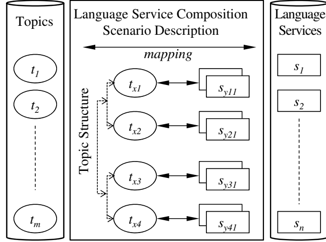
Figure 4.2: Scenario description aims at mapping proper language services to each topic
