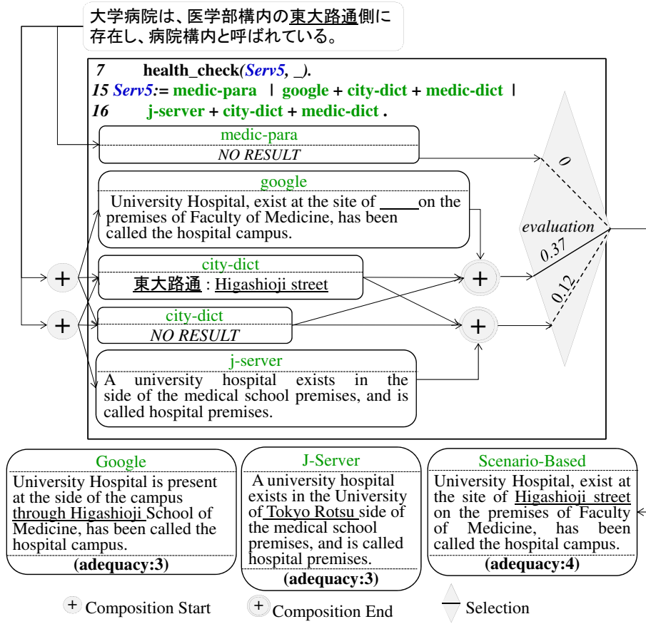
Figure 4.7: Integrating dictionary through composition ( health check topic)
