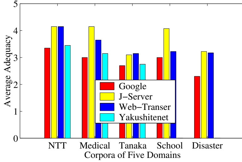
Figure 3.7: Average adequacy of each machine translation in five domains (adequacy is human score)
