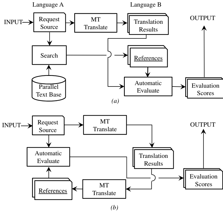
Figure 3.5: Two ways to prepare references (a) parallel text for reference preparation, (b) round trip translation way for reference preparation.
