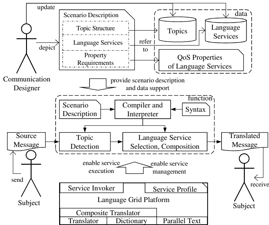
Figure 4.4: Architecture of scenario based language service composition
