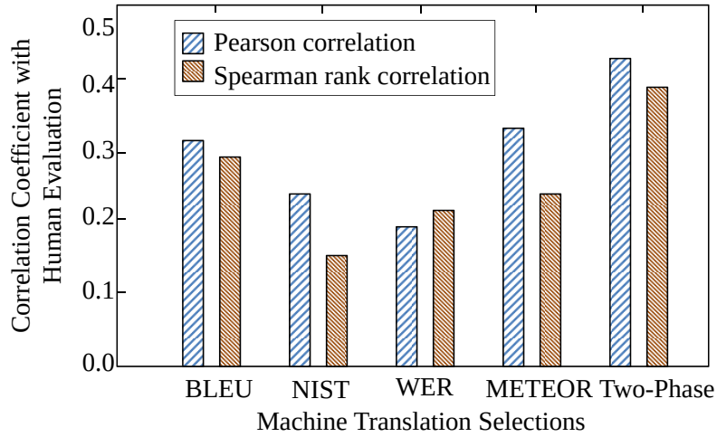
Figure 3.8: Correlation coefficient of machine translation selections
