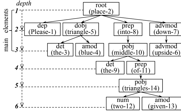
Figure 5.8: The tips for the repair strategy split ( the core of the message, which is the main elements of the sentence with low depth (less than 4) in the dependency structure tree. )
