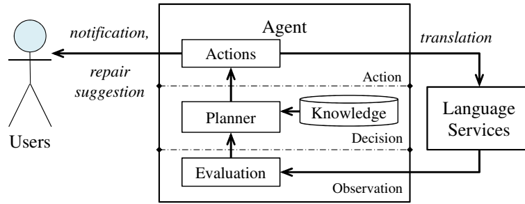
Figure 5.6: Architecture design of translation agent
