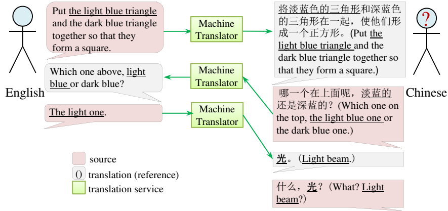
Figure 5.1: English-Chinese tangram arrangement communication ( the Chinese receives an inconsistent translated phrase and the communication breaks. )
