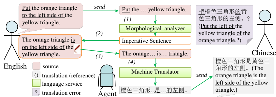
Figure 5.3: Interaction to handle mistranslated sentence
