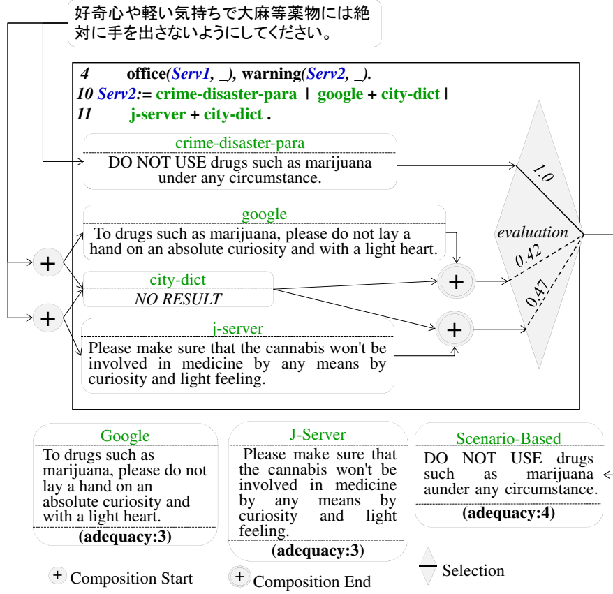
Figure 4.6: Integrating parallel text through selection (warning topic)
