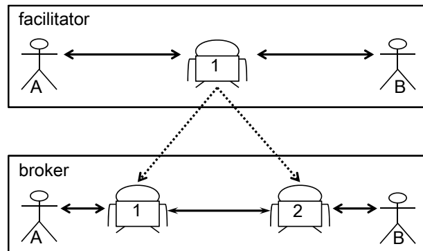
Figure 6.1: Two types of protocols: facilitator and adapter
