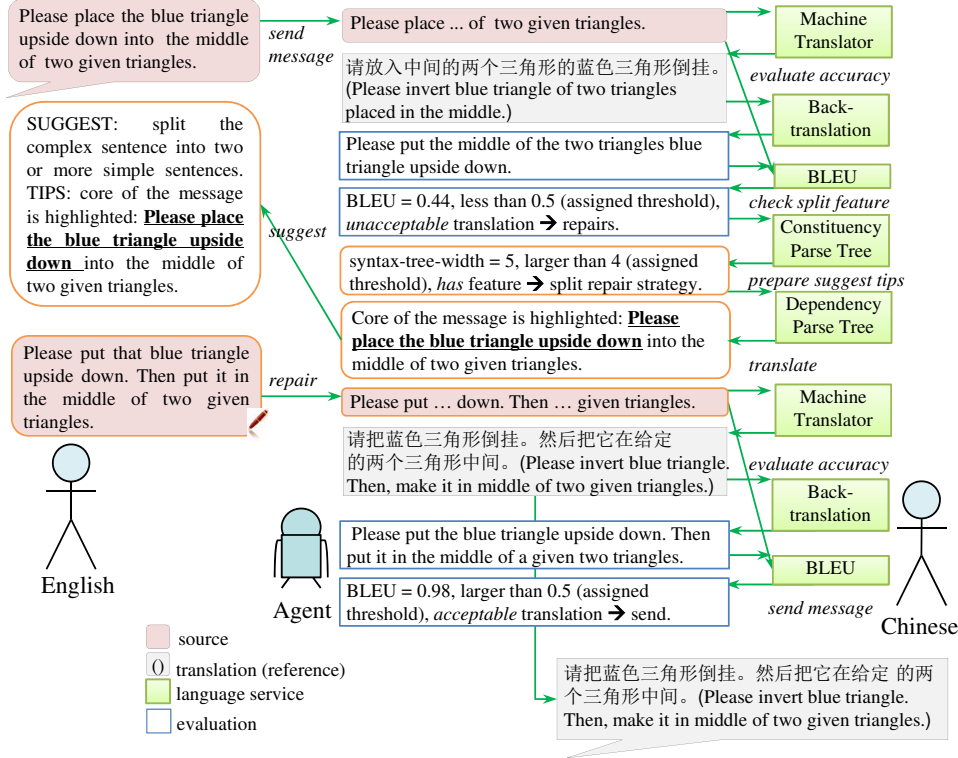
Figure 5.9: Example of agent's split strategy
