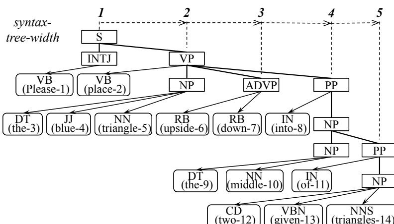
Figure 5.7: The syntax-tree-width feature of the repair strategy split ( a width of non-leaf part of its constituency structure tree.)
