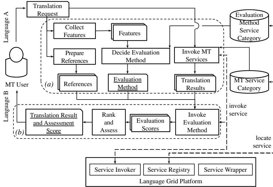
Figure 3.4: Architecture of machine translation service selection broker (a) selecting and preparing a proper evaluation method, (b) selecting a MT result and providing the assessment of selection.
