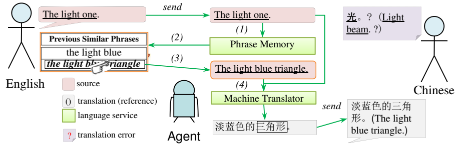
Figure 5.4: Interaction to handle inconsistently translated dialog (1) check the feature of similar phrases existing in previous dialog. (2) suggest selection of appropriate previous phrase. (3) choose a replacement of the previous phrase. (4) translate by the machine translator. )
