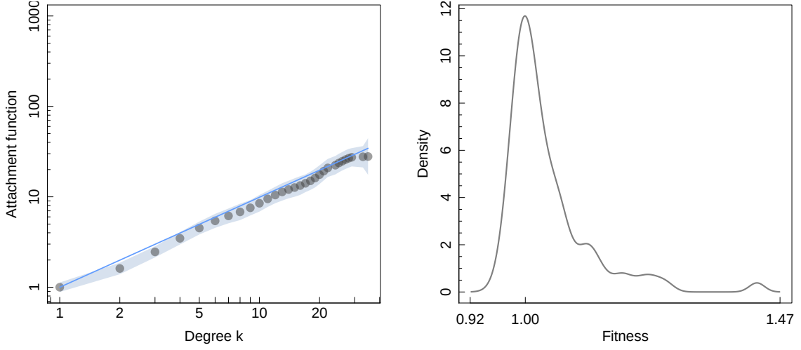
(a) Estimated A_k with joint estimation by PAFit ( \hat{\alpha} = 1.00 \pm 0.02 ). (b) Histogram of estimated node fitnesses.
