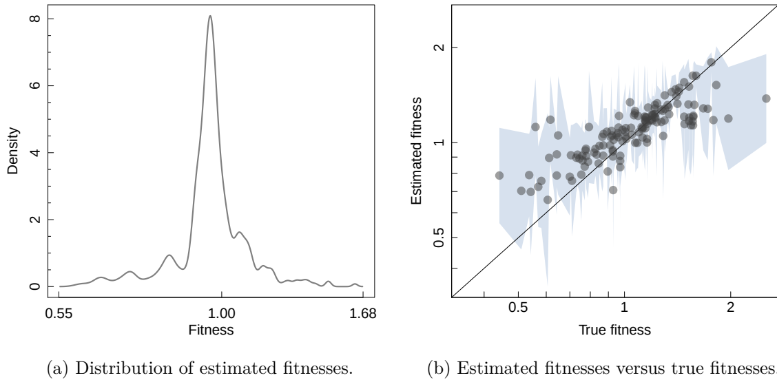
Figure 3: Estimating node fitnesses in isolation from sim_net_2 , which is generated with attachment function A_k = k . The true node fitnesses are sampled from a Gamma distribution with mean 1 and inverse variance 10. The attachment function in the estimation method is fixed at A_k = k . In panel b, we only plot nodes for which the number of acquired new edges is at least 5.
