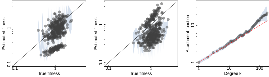
(a) Estimated and true \eta_i values when assuming A_k = k . \hat{s} = 2.7 . (b) Estimated and true \eta_i values when assuming A_k = 1 . \hat{s} = 4 . (c) Estimated PA function in isolation ( \hat{\alpha} = 0.57 \pm 0.02 ).
