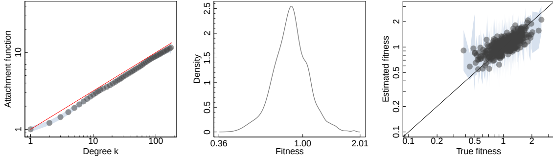
(a) Estimated attachment function ( \hat{\alpha} = 0.50 \pm 0.01 ). (b) Distribution of estimated node fitnesses. (c) Estimated and true \eta_i values.
