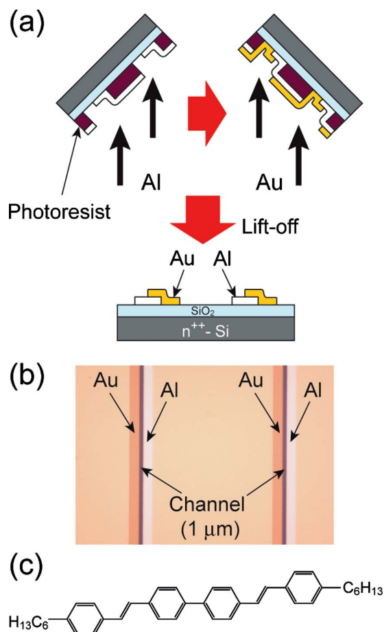
FIG. 1. (Color online) Preparation process for asymmetric contacts onto \text{SiO}_2/\text{Si} substrate (a). Optical micrograph of Au–Al contacts with channel length of 1\ \mu\text{m} (b). Molecular structure of BSBP-C6 (c).
