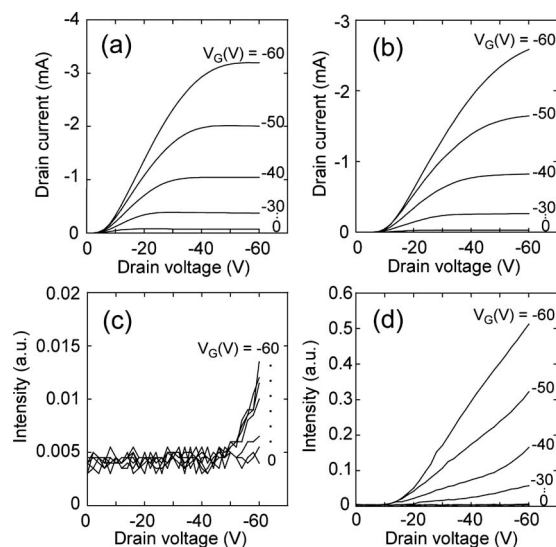
FIG. 2. FET [(a) and (b)] and emission characteristics [(c) and (d)] in 10\ \mu\text{m} channel length LE-OFETs. (a) and (c) show the results for a device with Au/Cr contacts. (b) and (d) show the results for a device with Au–Al contacts.
