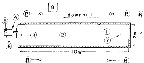
Fig. 1 A plan of the experimental catchment. 1—the boundary bricks, 2—the catchment area, 3—runoff water collector, 4—the runoff water tank, 5—the receiver of the rainfall intensity meter, 6—the cabinet of the water level recorder, 7—the plot for the temperature measurement, 8—the plot for the soil moisture measurement, P_1 \sim P_5 —the non-recording rain gages.
