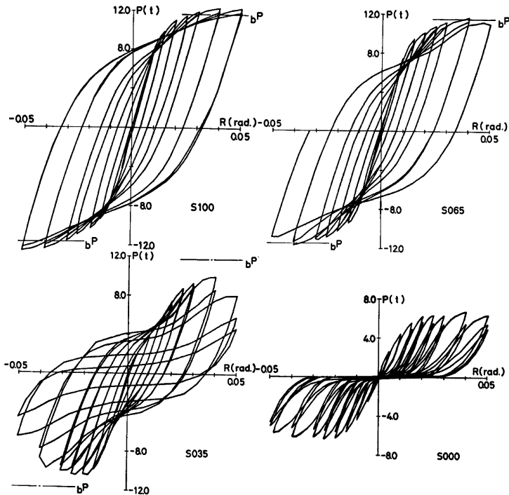
Fig. 3 Hysteresis loops.
