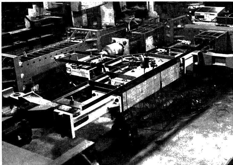
Photo. 2 Loading apparatus.
