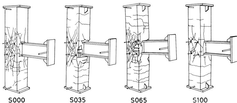
Fig. 2 Crack observation.
