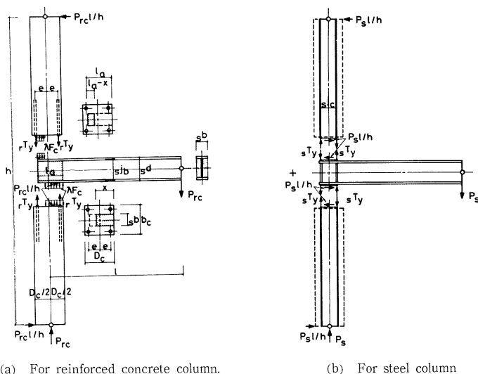
Fig. 4 Stress transfer mechanism.
