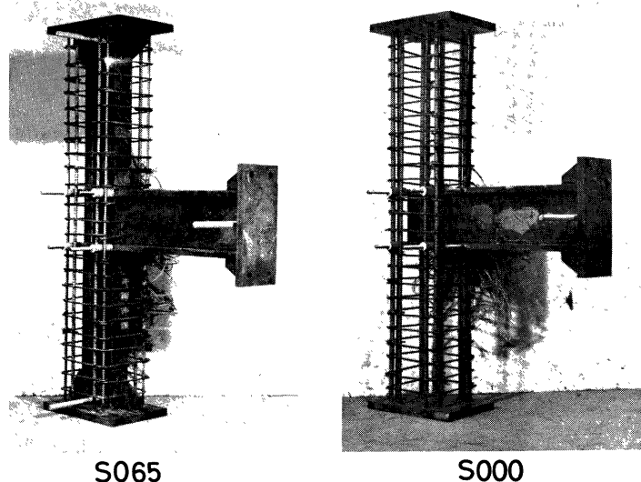
Photo. 1 Arrangement of reinforcement.
