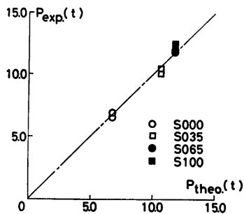
Fig. 9 Comparison of calculated values with experimental values.
