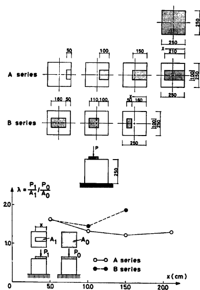
Fig. 8 Bearing capacity of the concrete block.
