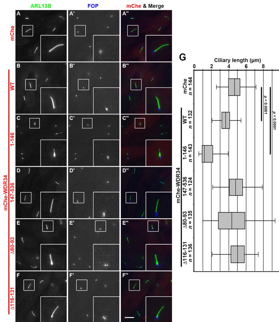
FIGURE 5: Expression of WDR34(1-146) in WDR34-KO cells inhibits ciliogenesis. The #W34-1-5 cell line stably expressing mChe (A), mChe-fused WDR34(WT) (B), WDR34(1-146) (C), WDR34(147-536) (D), WDR34( \Delta 80-93) (E), or WDR34( \Delta 116-131) (F) was cultured for 24 h under serum-starved conditions and double immunostained for ARL13B (A-F) and FOP (A'-F'). Scale bar, 10 \mu m. (G) Ciliary lengths of individual control cells and of the #W34-1-5 cell line expressing the WDR34 construct indicated were measured and are shown as box-and-whisker plots as described in the legend to Figure 3M.
