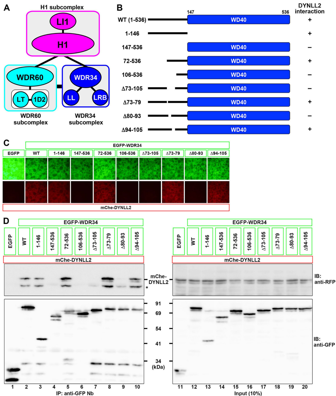
FIGURE 1: Region of WDR34 involved in DYNLL2 binding. (A) Schematic representation of the architecture of the dynein-2 complex predicted from our previous study (Hamada et al. , 2018). (B–D) Determination of the region of WDR34 involved in its interaction with DYNLL2. Lysates prepared from HEK293T cells cotransfected with expression vectors for an EGFP-fused WDR34 construct, as schematically shown in B, and mCh-fused DYNLL2 were immunoprecipitated with GST-tagged anti-GFP Nb prebound to glutathione–Sepharose beads, and subjected to the VIP assay (C) or immunoblotting analysis (D). IP, immunoprecipitation; IB, immunoblotting.
