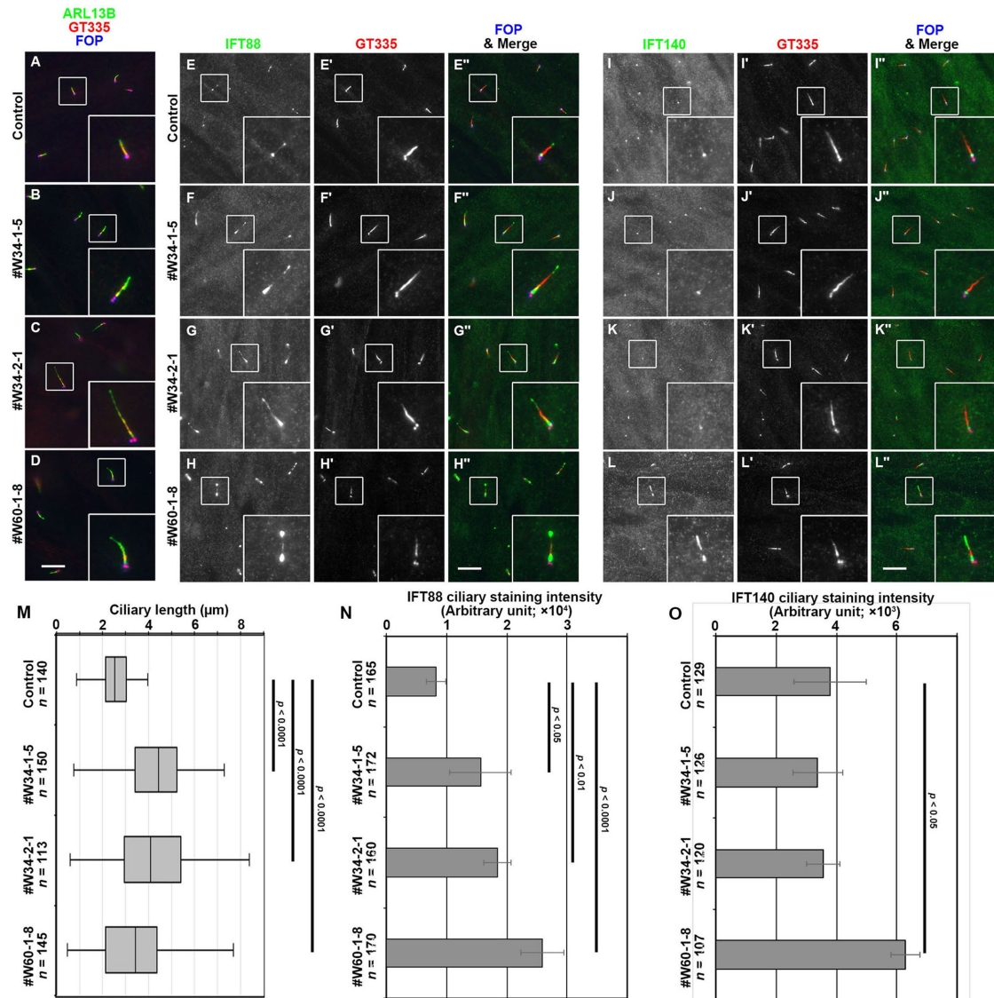
FIGURE 3: Accumulation of IFT88 within cilia in WDR34-KO cells. Control RPE1 cells (A, E, I), the WDR34-KO cell lines #W34-1-5 (B, F, J) and #W34-2-1 (C, G, K), and the WDR60-KO cell line #W60-1-8 (D, H, L) were serum-starved for 24 h to induce ciliogenesis, and triple immunostained with either an anti-ARL13B (A–D), anti-IFT88 (E–H), or anti-IFT140 (I–L) antibody, a GT335 antibody (A–D and E'–L'), which can react with polyglutamylated tubulins, and an anti-FOP antibody (A–D and E'–L'). Scale bars, 10 \mu m. (M) Ciliary lengths of individual control cells and of the WDR34-KO cell lines #W34-1-5 and #W34-2-1, and the WDR60-KO cell line #W60-1-8 were measured and are shown as box-and-whisker plots. The box represents the 25th–75th percentiles (interquartile region [IQR]) with the median indicated, and the whiskers show the minimum and maximum within 1.5 \times IQR from the 25th and 75th percentiles, respectively. The total numbers of ciliated cells analyzed (n) are shown. p , one-way analysis of variance (ANOVA) followed by Tukey post hoc analysis. (N, O) The staining intensity for IFT88 (N) or IFT140 (O) within cilia in control, WDR34-KO, and WDR60-KO cells were measured and are expressed as bar graphs. Values are means \pm SD of four (N) or three (O) independent experiments. In each experiment, 30–52 (N) and 33–52 (O) ciliated cells were observed, and the total numbers of ciliated cells observed (n) are shown. p , one-way ANOVA followed by Tukey post hoc analysis.
