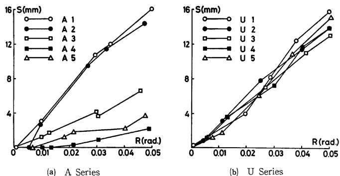
Fig. 10 Load-Slip Relationships
