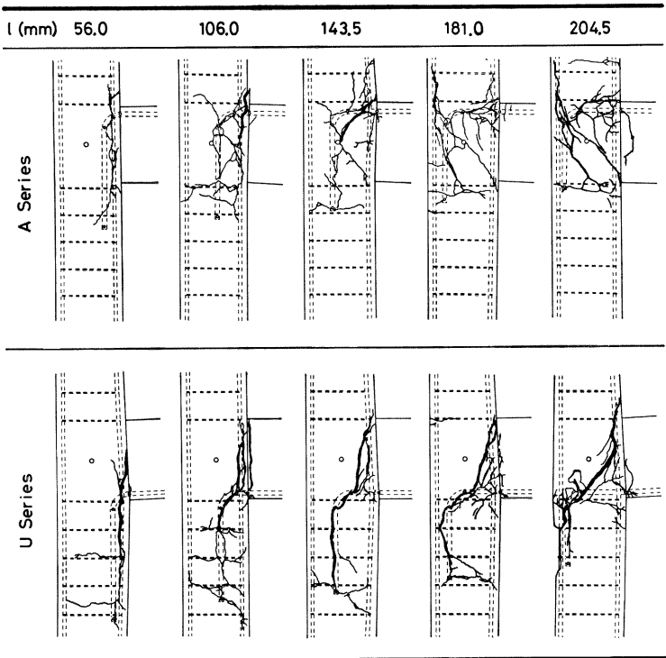
Fig. 7 Crack Observation of Exterior Joints
