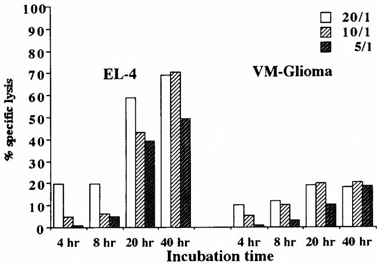
Fig. 10 Cytotoxicity mediated by resident macrophage (Mφ). Resident Mφ were obtained with peritoneal lavage of C3H/He mice. % specific lysis is expressed as mean of triplicate results from 3 independent experiments.
