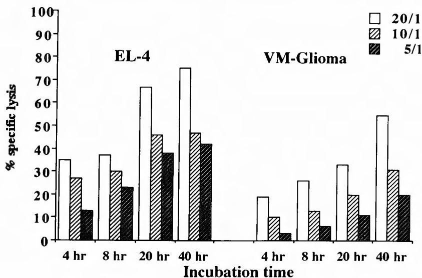
Fig. 12 Cytotoxicity mediated by activated macrophage (M \phi ). Activated M \phi were obtained from C3H/He mice following ip. injection of 200 \mu\text{g} lipopolysaccharide (LPS) 7 days prior to ^3\text{H} -TdR release-assay. % specific lysis is expressed as mean of triplicate results from 3 independent experiments.
