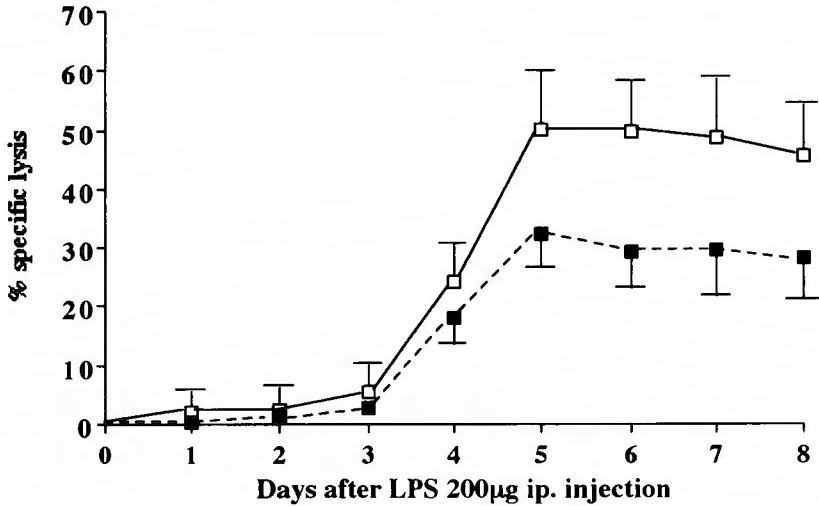
Fig. 1 Time course of killing activity of lipopolysaccharide (LPS)-activated macrophages (Mφ) against EL-4 (—□—) and VM-Glioma (---■---). Activated Mφ were obtained from C3H/He mice following ip. injection of LPS 200 μg between days 0 and 8 prior to 20 hr 51 Cr release-assay. % specific lysis is expressed as mean of triplicate results ± standard errors from independent experiments. Effector to target ratio of 20/1.
