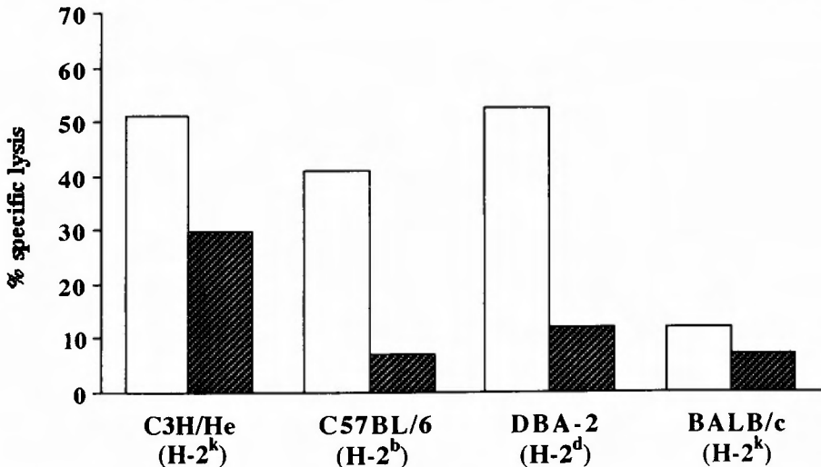
Fig. 2 Cytotoxicity of lipopolysaccharide (LPS)-activated macrophages (Mφ) derived from mice of 4 strains against EL-4 (H-2 k , □) and VM-Glioma (H-2 b , ▨) was not major histocompatibility complex (MHC) restricted. % specific lysis is expressed as men of triplicate results from 3 independent experiments. Effector to target ratio of 20/1.
