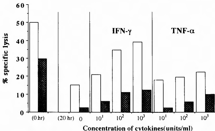
Fig. 6 Effects of interferon (IFN)- \gamma and tumor necrosis cfactor (TNF)- \alpha on the cytotoxicity of lipopolysaccharide (LPS)-activated macrophages (M \phi ) against EL-4 ( \square ) and VM-Glioma ( \blacksquare ). LPS-activated M \phi were cultured in vitro with IFN- \gamma or TNF- \alpha for 20 hr. % specific lysis is expressed as mean of triplicate results from 3 independent experiments. Effector to target ratio of 20/1.
