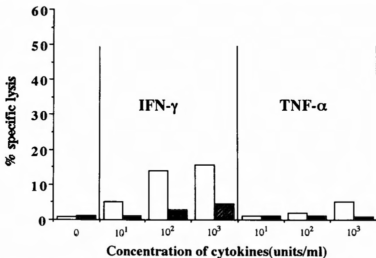
Fig. 3 Effects of interferon (IFN)- \gamma and tumor necrosis factor (TNF)- \alpha on the cytotoxicity of resident macrophage against EL-4 (□) and VM-Glioma (▨). Resident macrophages were obtained from C3H/He mice with peritoneal lavage. % specific lysis is expressed as mean of triplicate results from independent experiments Effector to target ratio of 20/1.
