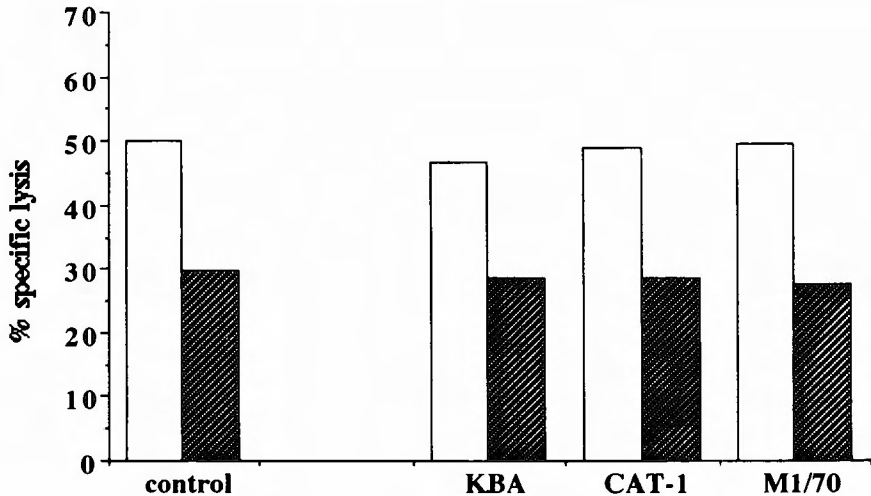
Fig. 9 Blocking effects of anti-adhesion molecules antibodies on the cytotoxicity mediated by lipopolysaccharide (LPS)-activated macrophages (Mφ) against EL-4 (□) and VM-Glioma (▨). Anti-lymphocyte functioning antigen (LFA)-1 antibodies (KBA, 1/20 diluted ascites fluid), anti-intracellular adhesion molecule (ICAM)-1 antibodies (CAT-1, 1/20 diluted ascites fluid), and anti-Mac-1 (M1/70, 1/20 dilution) were added during 20 hr 51 Cr release-assay. % specific lysis is expressed as mean of triplicate results from 3 independent experiments. Effector to target ratio of 20/1.
