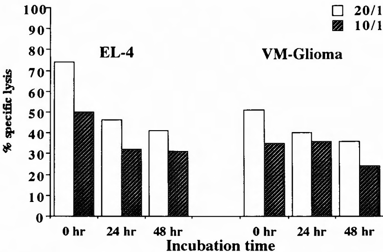
Fig. 13 Kinetics of spontaneous decrease in killing activity of activated macrophage (Mφ) following initiation of in vitro culture. Lipopolysaccharide (LPS)-activated Mφ were assayed for their ^3\text{H} -TdR release-assay at 0, 24, and 48 hr after initiation of in vitro culture. % specific lysis is expressed as mean of triplicate results from 3 independent experiments.
