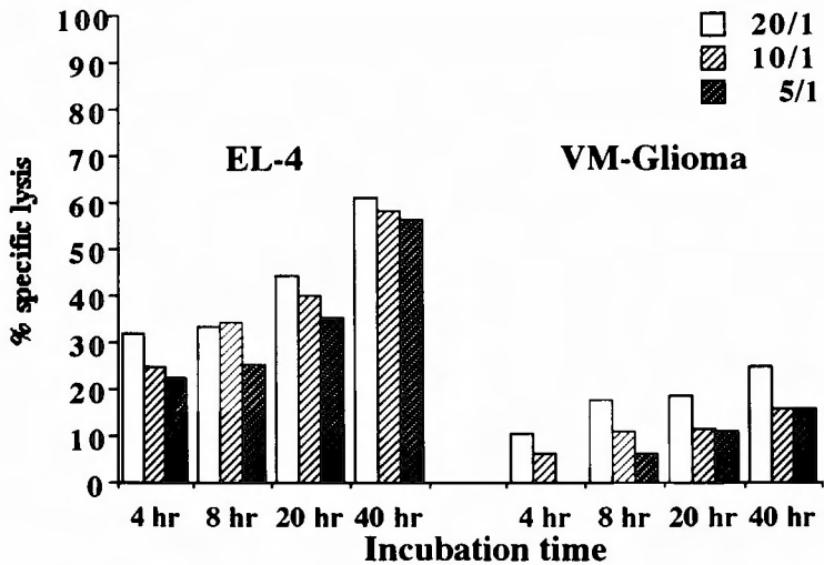
Fig. 11 Cytotoxicity mediated by elicited macrophage (Mφ). Elicited Mφ were obtained from C3H/He mice following ip. injection of 2 ml thioglycollate 4 days prior to 3 H-TdR release-assay. % specific lysis is expressed as mean of triplicate results from 3 independent experiments.
