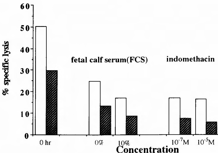
Fig. 7 Effects of fetal calf serum (FCS) and indomethacin on the cytotoxicity of LPS-activated macrophages (M \phi ) against EL-4 (□) and VM-Glioma (▨). LPS-activated M \phi were cultured in vitro with FCS or indomethacin for 20 hr. % specific lysis is expressed as mean of triplicate results from 3 independent experiments. Effector to target ratio of 20/1.
