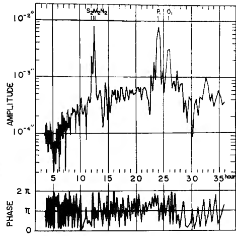
Fig. 12. Amplitude and phase spectra of the N-S ( B_E ) at Akibasan.
