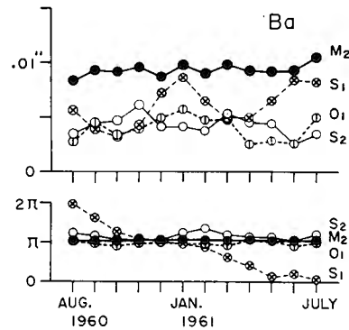
Fig. 9f. N-S component tilt at Akibasan.
