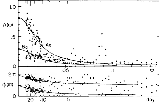
Fig. 18. Ratios of the corrected spectra of the ground tilts to the spectrum of intensity of precipitation. Open and solid circles are the results for the E-W and N-S component tilts respectively. Solid curves denote the amplitude and phase spectra of the impulse responses, h_E(t) and h_N(t) .
