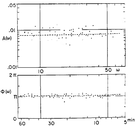
Fig. 16a. Amplitude ratio and phase difference of the E-W component tilt at Oura to the atmospheric pressure. Unit of the ordinate of the ratio is second of arc/mb.
