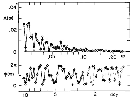
Fig. 13. Spectral amplitude A(\omega) and phase \phi(\omega) of the E-W component tilt at Akibasan. The cross represents the corrected values for the oceanic tides, air temperature, atmospheric pressure and its time derivative.
