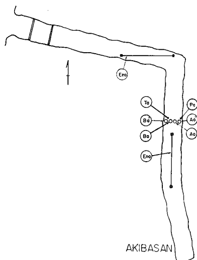
Fig. 2b. Configuration of instruments at the Akibasan station.
