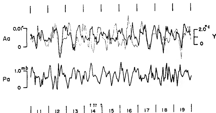
Fig. 32. Comparison of the filtered results of the E-W component tilt at Akibasan ( A_a ) with those of the air temperature ( Y , dashed line) and atmospheric pressure P_a . The response of the used filter is 1 in the periodic ranges from 1 to 11.5 hours and from 13.6 to 22.5 hours.
