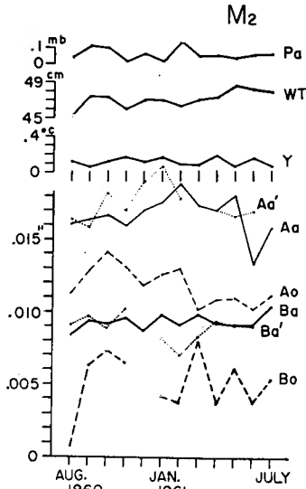
Fig. 10 a. Comparison of the amplitudes in respect of the M_2 constituent.
