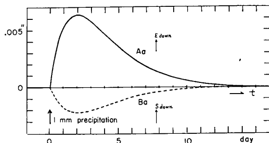
Fig. 19. Response of the ground tilts at Akibasan by an impulsive precipitation.
