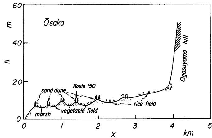
Fig. 15. Land utilization and topography in the east area of the Kiku river.
