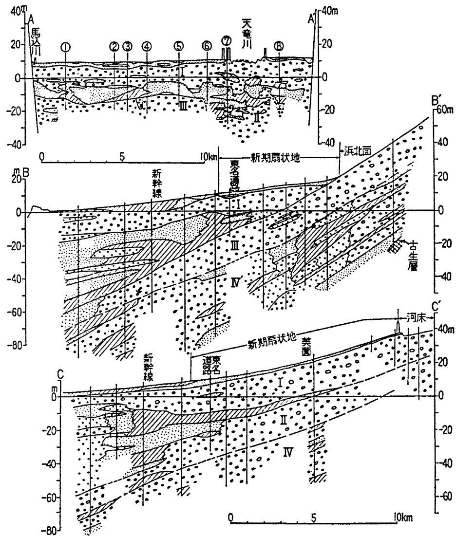
Fig. 7. Geological section of Tenryu alluvial fan 1)
