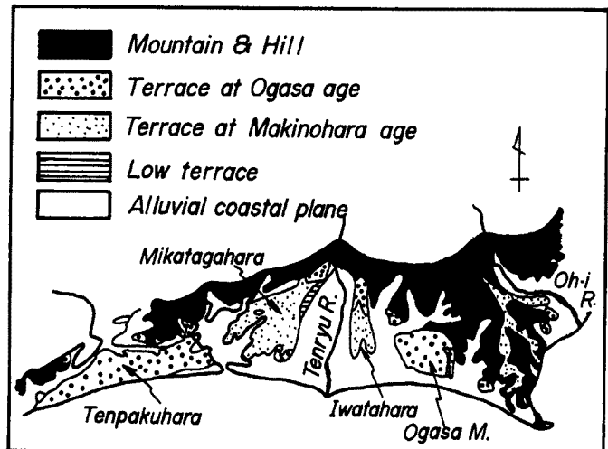
Fig. 19. Distribution of hills and plateaus 6)
