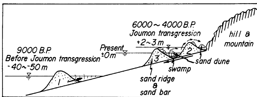
Fig. 17. Schematic diagram of development of beach ridge, sand dune and sea-level changes.
