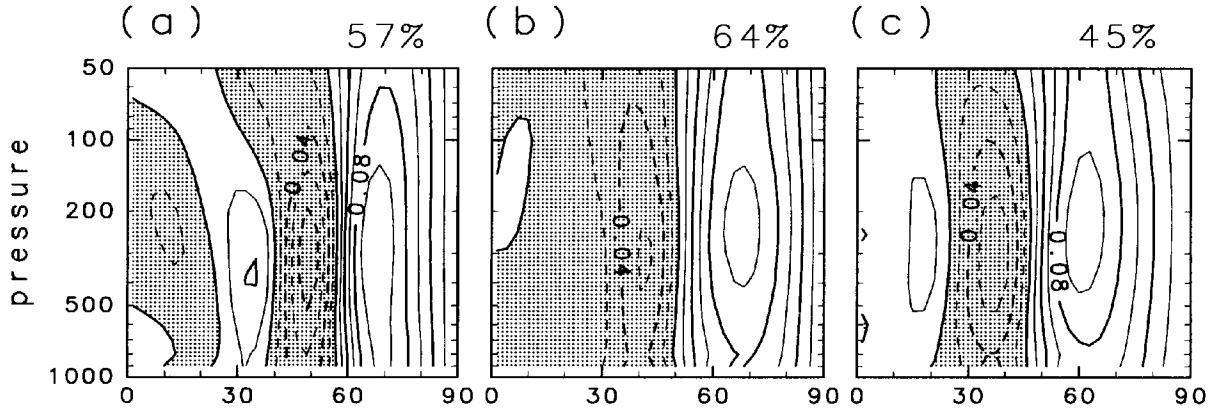
Fig. 5: EOF1 of zonal mean zonal wind in (a)FLAT, (b)WN1 and (c)WN2 experiments. Number on the top right corner in each panel represents contribution rate.
