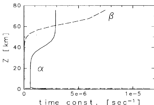
Fig. 2: Relaxation time constant for Newtonian cool/heating ( \alpha ) and Rayleigh frection ( \beta ).
