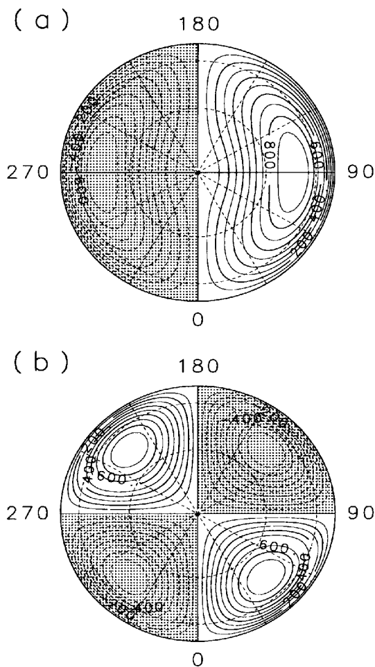
Fig. 3: Topography in (a) WN1 and (b) WN2 experiments. Negative value is hatched. Outside numbers show longitude.
