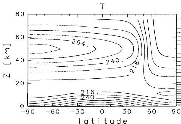
Fig. 1: Radiative equilibrium temperature for Newtonian cool/heating. Horizontal lines on the right-hand side denote the positions of vertical discretization and dashed lines are those for bottom boundary layer and for top sponge layer.
