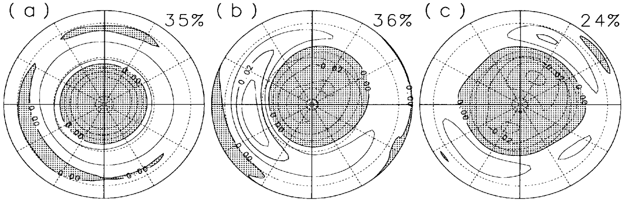
Fig. 4: EOF1 of surface pressure in (a)FLAT, (b)WN1 and (c)WN2 experiments. Number on the top right corner in each panel represents contribution rate.
