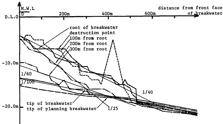
Fig. 2. Sea bottom profiles of Shingu Harbor.
