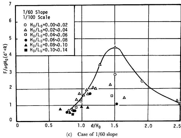
Fig. 10. Relation between non-dimensional wave force F/\rho g H_0(d'+R) and relative depth d/H_0 by authors' experiments.
