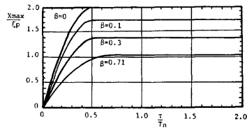
Fig. 6. Response spectra to rectangular pulse (after Goda 1) ).
