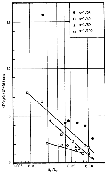
Fig. 11. Relationship between non-dimensional wave force F/\rho g H_0(d'+R) max and deep water wave steepness H_0/L_0 .
