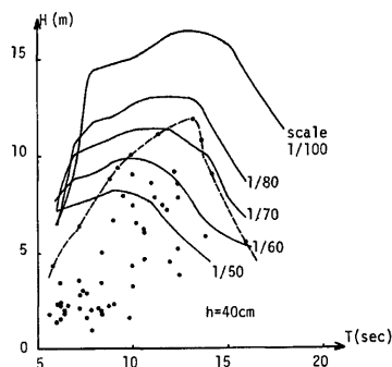
Fig. 4. Distribution of Maximum wave height and period at Shingu Harbor and characteristics of wave generator used in model experiments.
