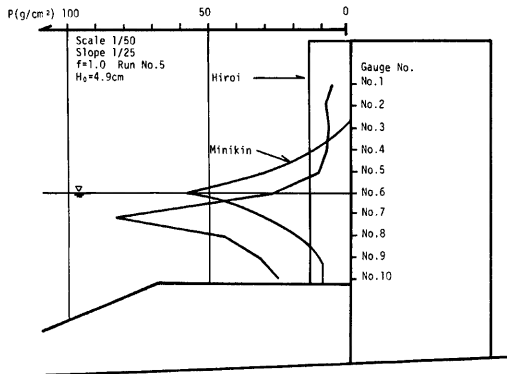
Fig. 8. Vertical distribution of wave pressure.
