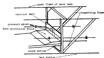
Fig. 5. Schematic illustration of model equipment (water depth 40 cm).
