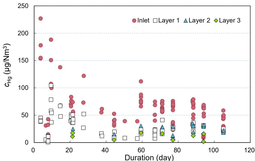
Figure 4-15. The concentrations of Hg^0 in the inlet and outlet of the polymer tower at C-F.
