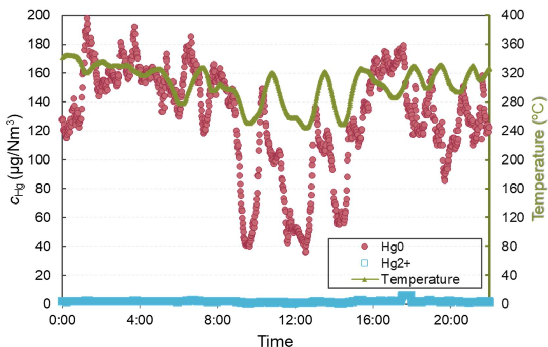
Figure 4-12. Concentrations of \text{Hg}^0 and \text{Hg}^{2+} in the pyrolysis gas and the temperature in C-F.
