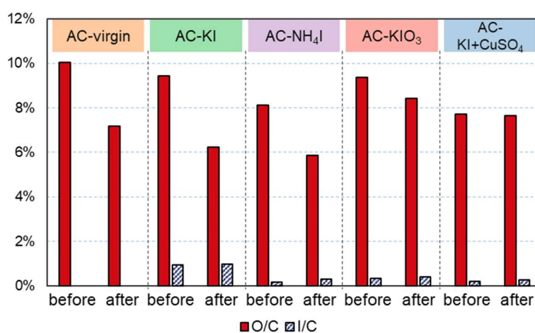
Figure 5-5. Surface elemental composition derived from wide-scan analysis (based on atomic concentration). After adsorption, the ratio of I/C in impregnated ACs increased due to the decrease in the amount of C. Additionally, the O/C ratio decreased for all sorbents except AC-KI+CuSO 4 , which implies that the amount of O also decreased after adsorption. These results indicate that C and O were consumed during chemisorption of Hg 0 . Further, the decreased C and O on the surfaces of the sorbents suggests that a gaseous phase product—possibly CO 2 —might have formed and escaped into the carrier gas during this process (Eichberger and Stieglitz, 1994).
