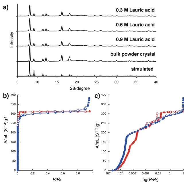
Figure 2. a) PXRD patterns of as-synthesized bulk and nanocrystals of 1 . The simulated patterns are obtained from the single-crystal structure. b) Nitrogen adsorption (solid circle) and desorption (open circle) isotherms of at 77 K of bulk (red) and the smallest nanocrystals obtained with the condition of 0.3 M lauric acid (blue) of 1 . c) Sorption isotherms plotted on a logarithmic scale. STP is standard temperature and pressure.
