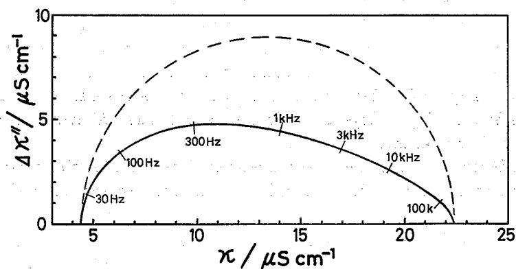
Fig. 3. Complex plane plots of \kappa and \Delta\kappa'' = 2\pi f\epsilon_0(\epsilon - \epsilon_n) with the same data as shown in Fig. 1.
