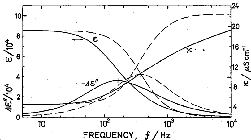
Fig. 1. Frequency dependence of the relative permittivity \epsilon , the electric conductivity \kappa and the loss factor \Delta\epsilon'' = (\kappa - \kappa_i)/(2\pi f \epsilon_v) calculated from Hanai's Eq. (12). The phase parameters used: \epsilon_a = 2.1 , \kappa_a = 6.55 \times 10^{-5} \mu\text{S cm}^{-1} , \epsilon_i = 77.5 , \kappa_i = 24.5 \mu\text{S cm}^{-1} and \phi = 0.98 . Dashed curves are single relaxation profiles with the same values of \epsilon_i , \epsilon_h , \kappa_i and \kappa_h as calculated from Eq. (12).
