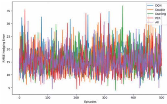
Figure 2: Hedging error for 2 hidden layers and 500 episodes
