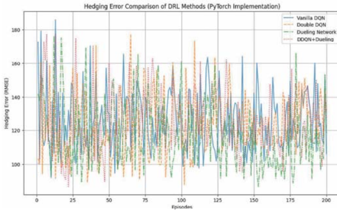
Figure 3: Hedging error for 5 hidden layers and 200 episodes
