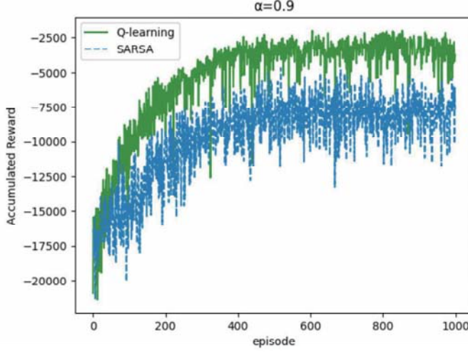
Figure 1: Stability and Convergence of Q-learning and SARSA Learning at a Learning Rate of \alpha = 0.9
