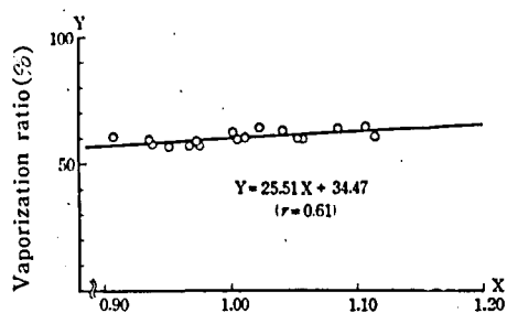
Fig. 1. Effect of burning rate on vaporization ratio of allethrin from burning mosquito coil (0.60% of (\pm) - cis,trans -allethrin)
