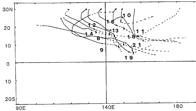
Fig. 8 (a). Trajectories of cyclonic disturbances which became typhoons in the period from July to October in 1980. \phi marks denote the place where they became Tropical Depressions and white circles denote the place where they became Tropical Storms. Numerals denote numbers of typhoons.
