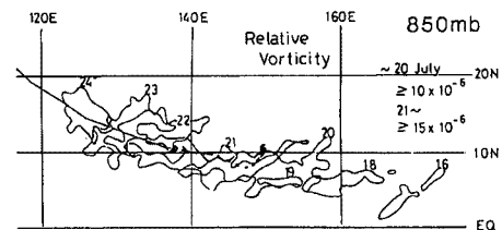
(e) The time change of the position of 850 mb-level positive relative vorticity. Before 20 July, larger than 10 \times 10^{-6} \text{ sec}^{-1} regions are drawn and larger than 15 \times 10^{-6} \text{ sec}^{-1} after 21 July.
