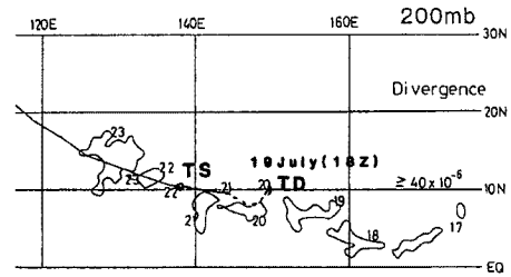
(c) The time change of the position of 200 mb-level divergent region (larger than 40 \times 10^{-6} \text{ sec}^{-1} ) at 00Z, which relates to Typhoon KIM (8009). Solid line indicate the trajectory of the typhoon.
