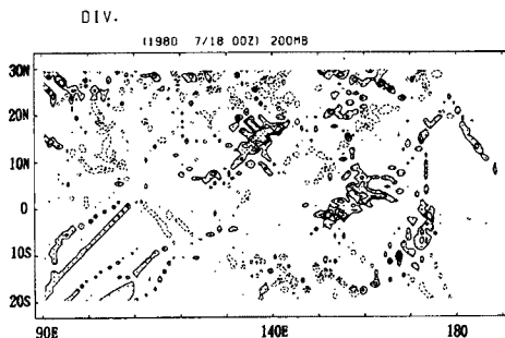
Fig. 7(a). 200 mb-level horizontal divergence field at 00Z on 18 July 1980. Contour interval is 20 \times 10^{-6} \text{ sec}^{-1} and larger than 20 \times 10^{-6} \text{ sec}^{-1} area are shaded.
