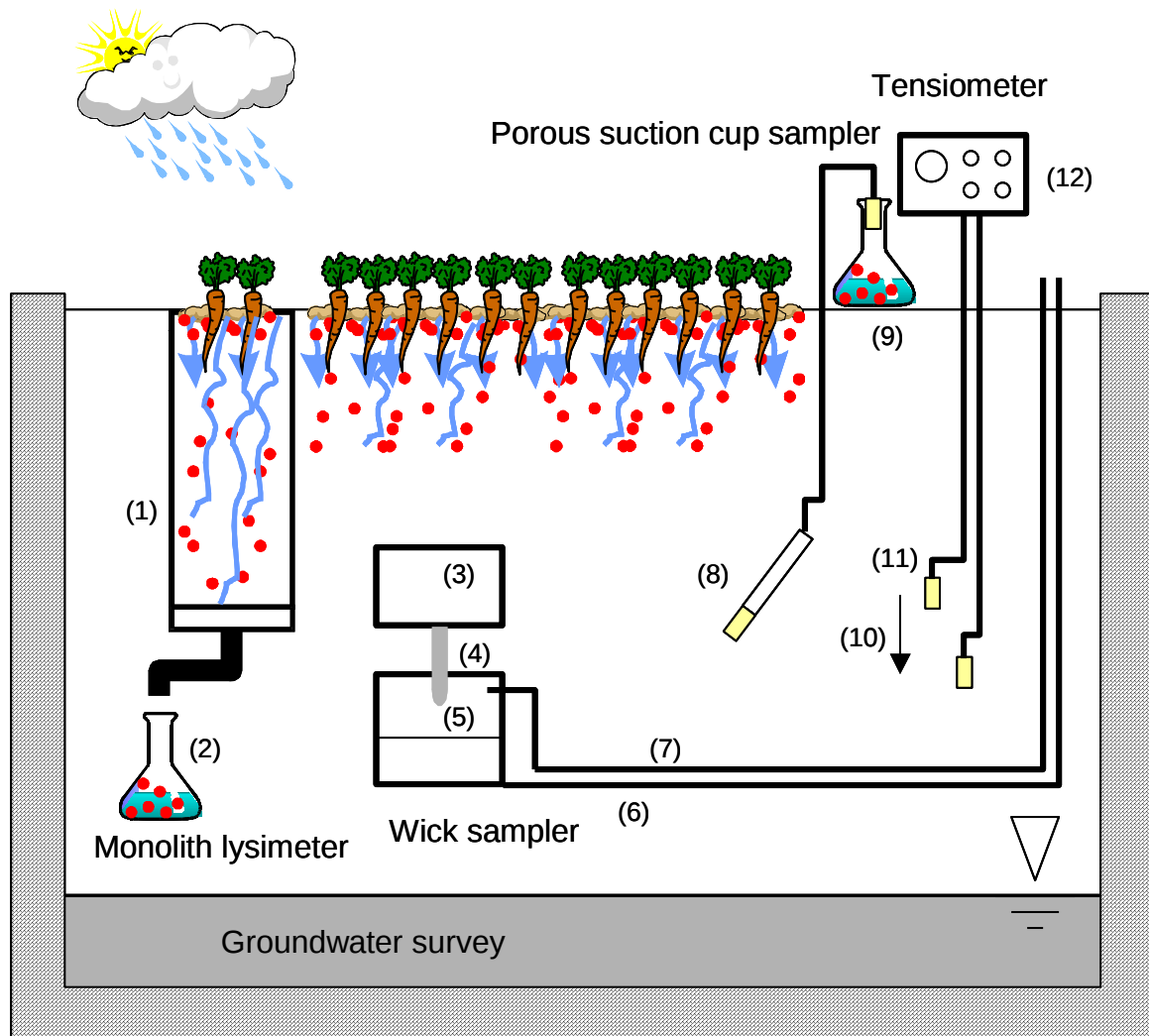
Lysimeter facility
