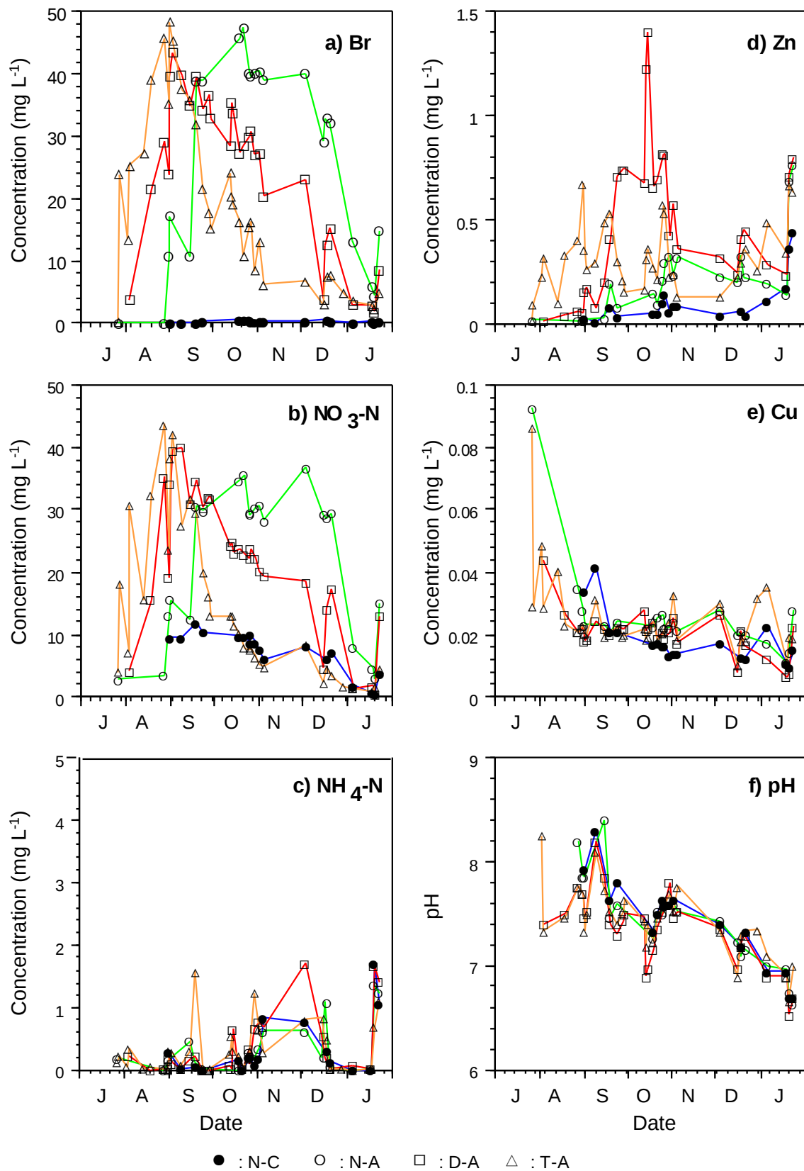
Fig. 5.6. Concentrations of a) Br, b) NO 3 -N, c) NH 4 -N, d) Zn, and e) Cu, and f) pH values in leachate during the period 22 July 1998 to 25 January 1999. Each value represents the mean of three replicates.
