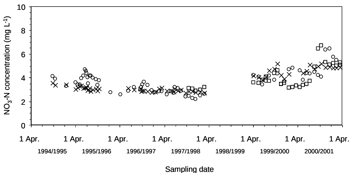
Fig. 4.3. Nitrate N concentration in groundwater in two plots receiving ammonium fertilizer (□; ○) and one plot without fertilizer (×), from 1994 to 2001.
