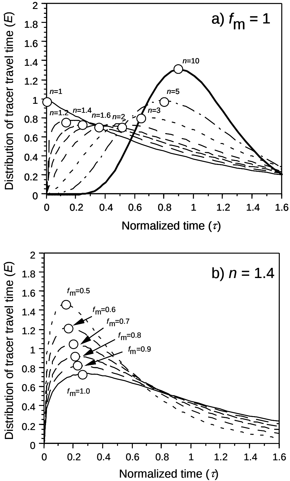
Fig. 5.1. Sensitive analysis of the parameters n and f_m used in the modified tanks-in-series model. a) Change of n in case of f_m = 1 ; and b) change of f_m in case of n = 1.4 . The peaks of E(\tau) are marked with a circle.
