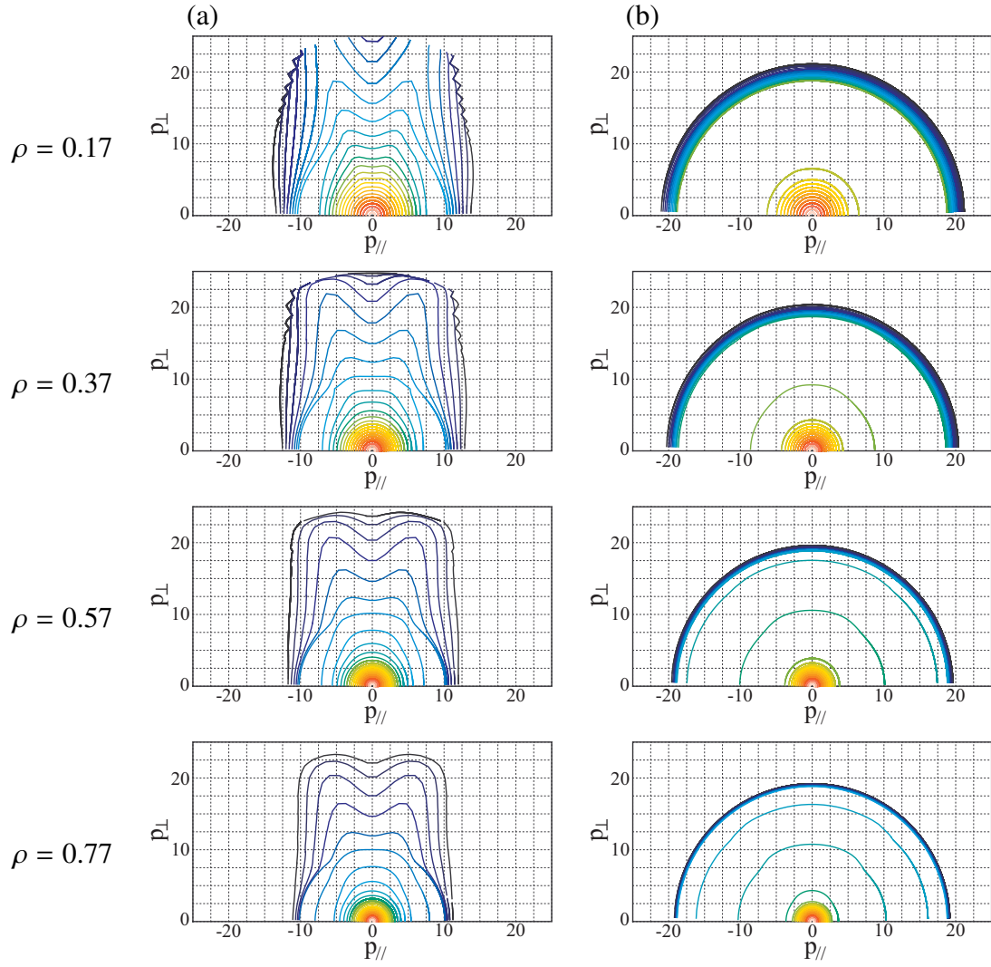
Figure 6.2: The contour of the momentum distribution functions of triton and helium ion in 2D momentum space at several radial points are shown.
