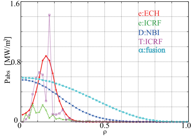
Figure 5.4: The power absorption profiles of ECH, ICRF, and NBI for each species. ICRF absorption profiles for electron (green) and triton (purple) are calculated using the wave electric field calculated by TASK/WM. These heat profiles are fixed in time during the simulation of this chapter. The absorption powers for NBI, ICRF, and ECH are 31.6MW, 20.5MW, and 20.4MW, respectively. ICRF absorption power consists of 4.72MW for electron and 15.8MW for triton. In this figure, the only \alpha particle source power varies in time.
