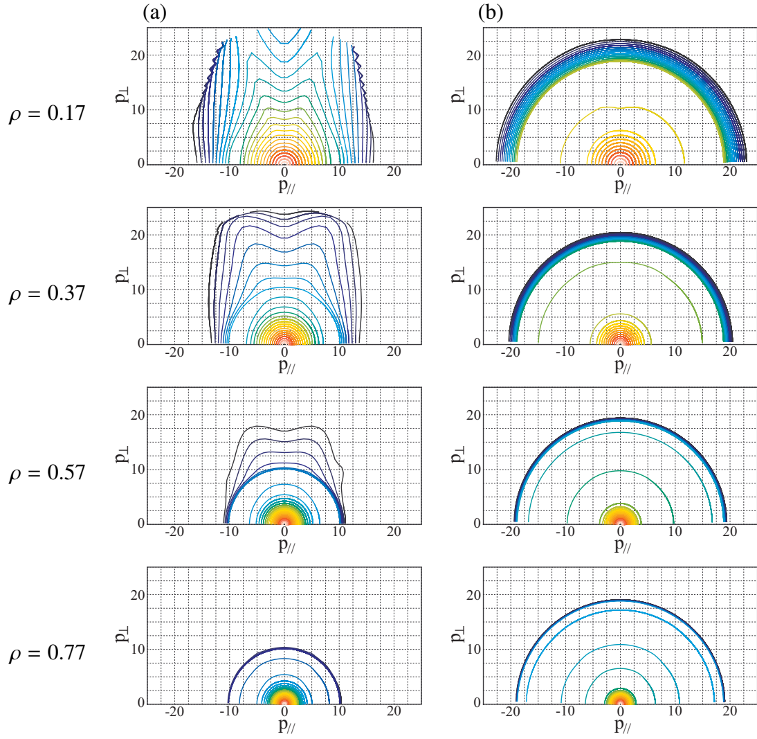
Figure 6.11: The contour of the momentum distribution functions of triton and helium ion in 2D momentum space at several radial points are shown.
